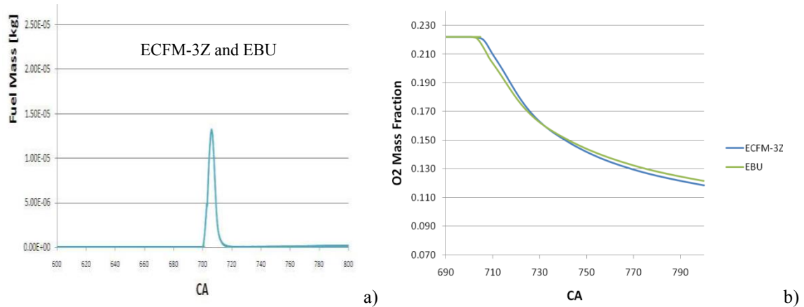
Figure 3. Comparison of Fuel mass and O 2 mass fraction for both of models a) Fuel mass & CA, b) O 2 mass fraction & CA
