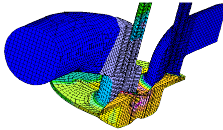
Figure 4. Sectional mesh view for full geometry
