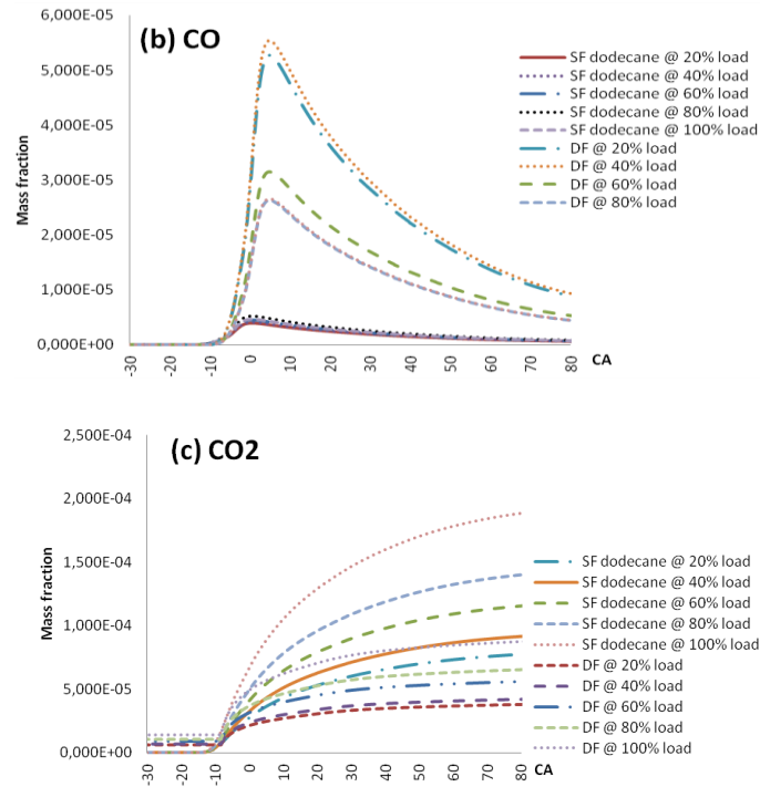
Figure 8. Exhaust emissions for single and dual fuel cases with different engine loads
