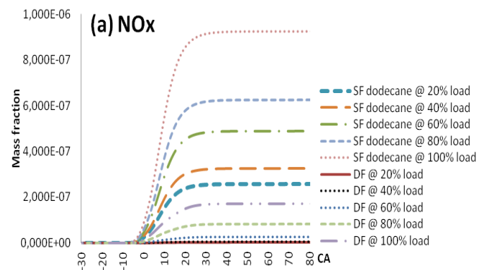
Figure 7. NOx for single and dual fuel cases versus CA.
