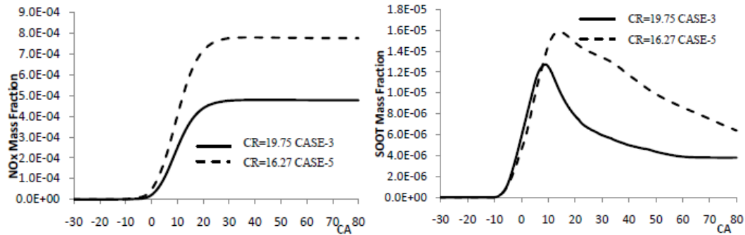
Figure 12. Comparison of the best PPCI cases according to emission performance for different compression ratio
