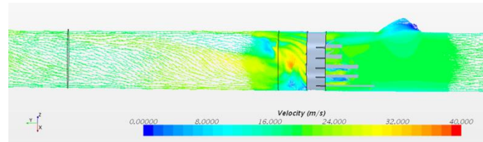
Figure 14. Velocity vector at the cone k-epsilon
