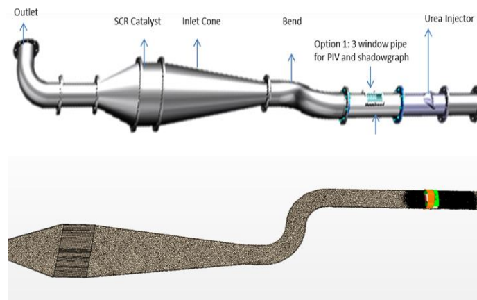
Figure 5. SCR Aftertreatment inline model and computational domain
