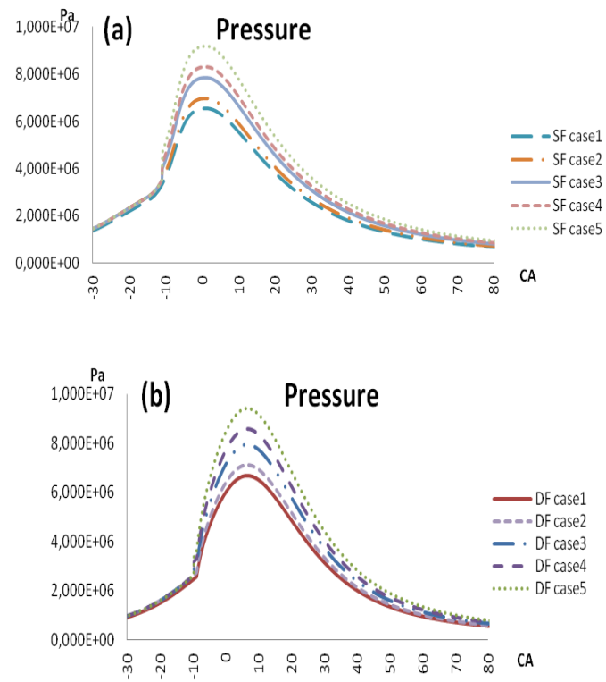
Figure 6. Combustion characteristics at different engine load. (a) Single fuel (dodecane) cases. (b) Dual fuel (CBG+dodecane) cases.
