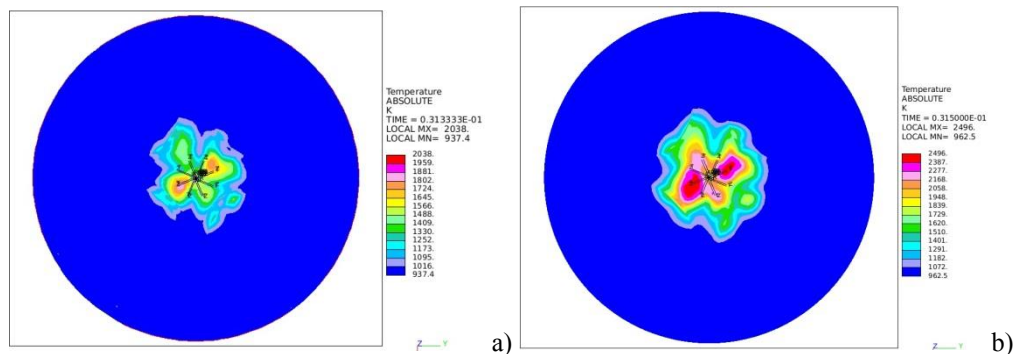
Figure 2. Temperature contours perpendicular to the vertical axis at 0.16 mm below from cylinder head a) 10 °CA bTDC for EBU, b) 10 °CA bTDC for ECFM-3Z
