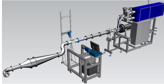
Figure 9. Schematic of exhaust system layout with emission
