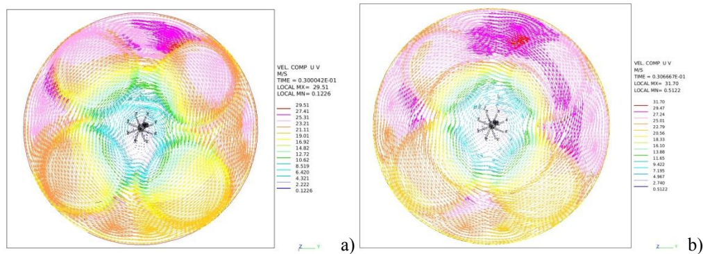
Figure 1. Velocity vector fields perpendicular to the vertical axis at 0.16mm below from cylinder head a) 20 °CA bTDC for EBU, b) 20 °CA bTDC for ECFM-3Z
