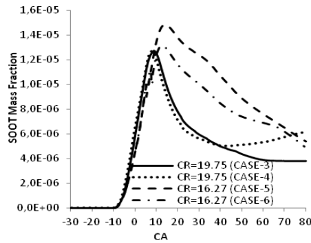
Figure 13. Effects of the compression ratio on the emissions.
