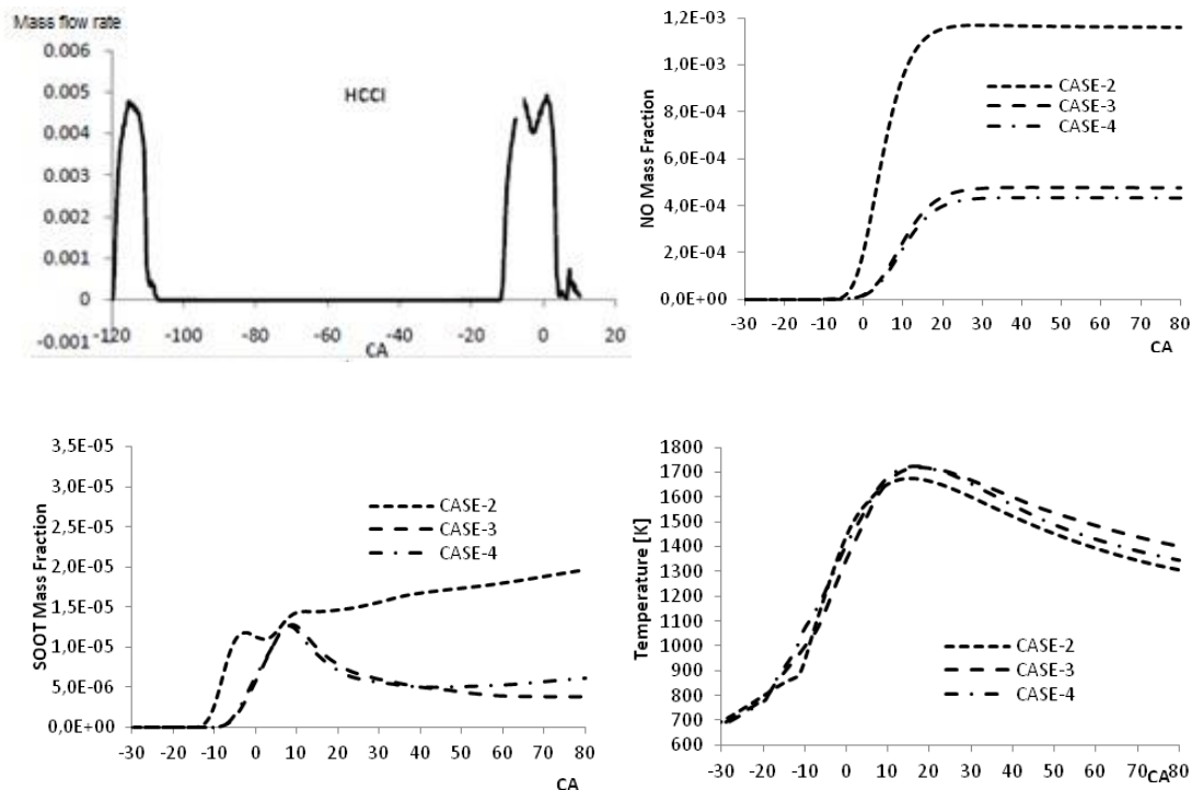
Figure 11. Comparison of the results for different the spray angles
