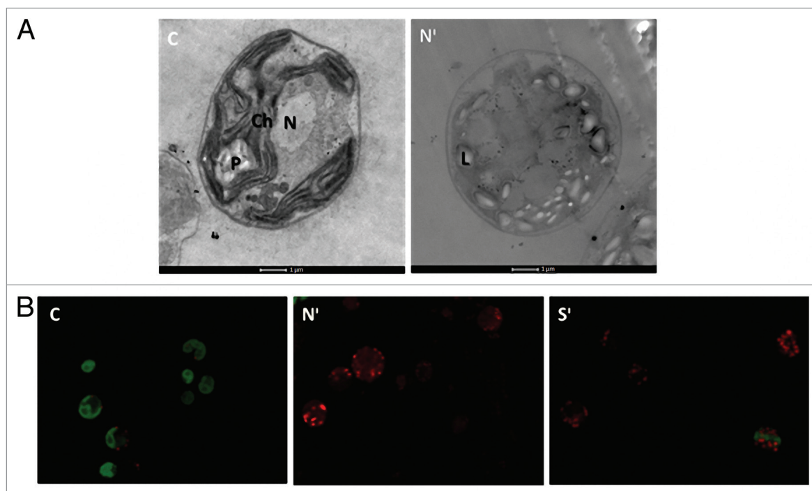
Figure 1. Transmission electron microscopy (A) and confocal fluorescence microscopy (B) images of control, N-starved and S-starved C. reinhardtii cells sampled on fifth day of incubation. In the fluorescence images green represents chlorophyll autofluorescence and light red represents Nile red fluorescence. Abbreviations: C, control; N', N-depleted cells; S', S-depleted cells; Ch, chloroplast; P, pyrenoid; N, nucleus; L, lipid bodies.
