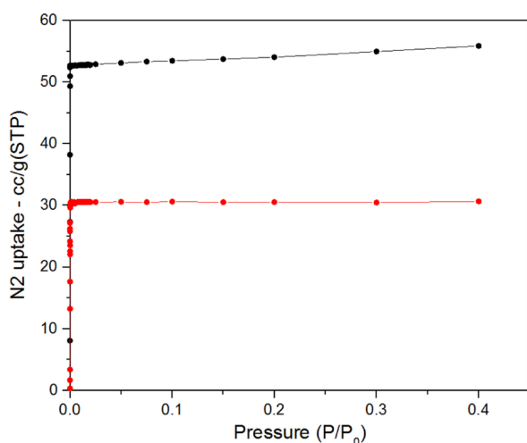
Figure 4. Simulated N 2 isotherms at 77 K in 1 (black) and 2 (red).
