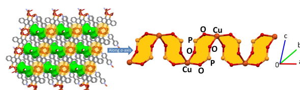
Figure 1. The 3D structure of 1 , showing the voids highlighted in green within the framework and 1D SBU composed of edge sharing Cu-O-P-O-Cu-O-P-O rings.
