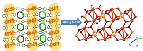
Figure 2. The 3D structure of 2 , showing the voids highlighted in green within the framework and 1D SBU with edge sharing Cu-O-P-O rings, and the central bridging \{\text{Cu}_2\text{O}_2\} rhombi.
