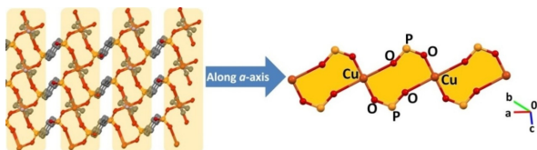
Figure 3. The 3D framework of 3 , edge sharing Cu–O–P–O–Cu–O–P–O rings.
