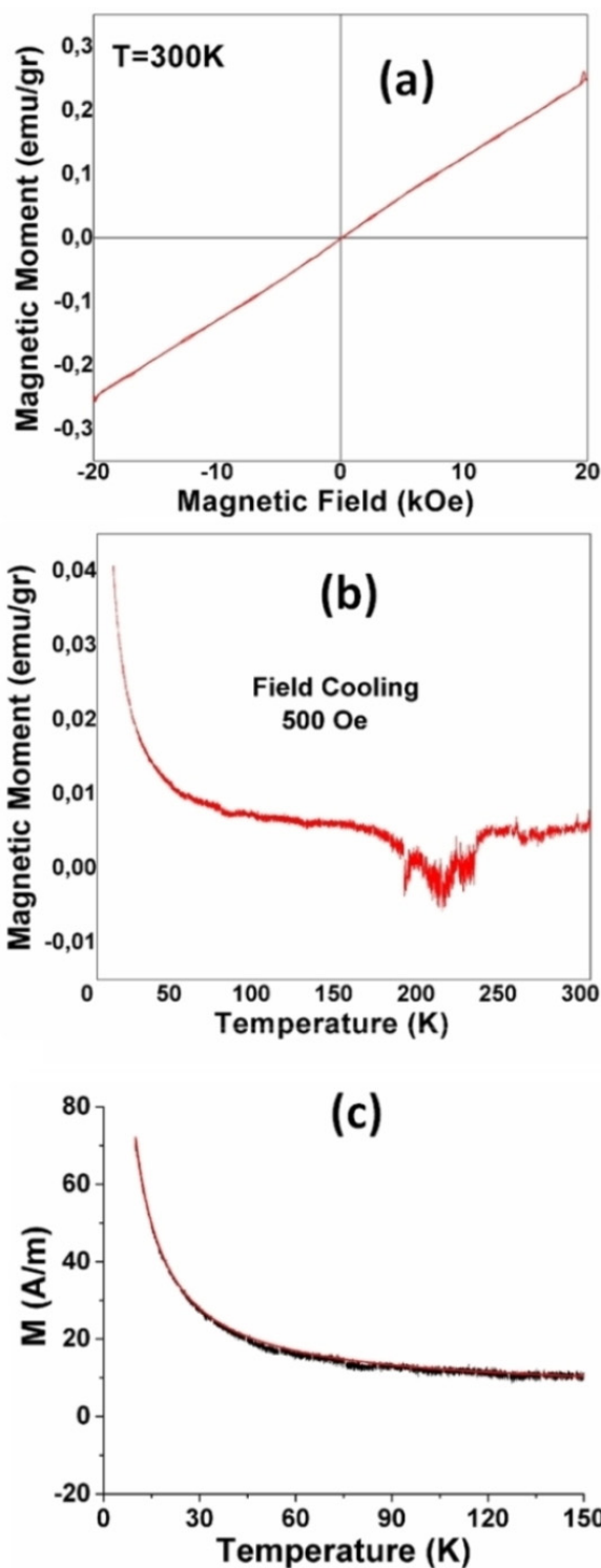
Figure 5. (a) Magnetization measurement of 1 showing paramagnetic behavior at 300 K (b) Magnetization vs. temperature with a dc field cooling from 300 K at 500 Oe (c) Curie Law fitting of the curve from 10–150 K.
