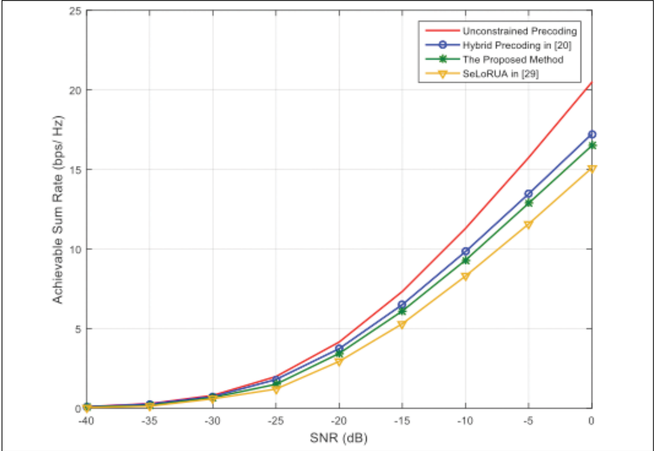
Figure 1. Achievable sum rate versus SNR
