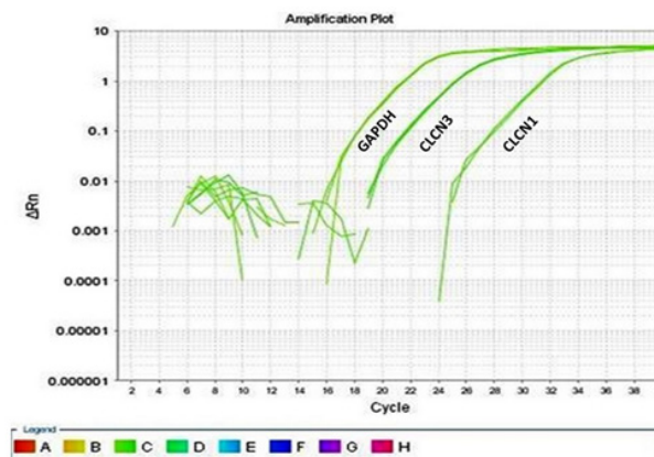
Fig. 2. Real-time PCR amplification plot for control samples is displayed on a graph, with cycle number on the x-axis and change in fluorescent intensity ( \Delta Rn ) on the y-axis. CLCN3 has a Ct number of 22 and CLCN1 has a Ct number of 28, with CLCN3>CLCN1 for \Delta Rn 0.1. GAPDH: Glyceraldehyde 3-phosphate dehydrogenase. CLCN3: Chloride Voltage-Gated Channel 3 (CLIC-3)(4q33). CLCN1: Chloride Voltage-Gated Channel 1 (CLIC-1) (7q35).
