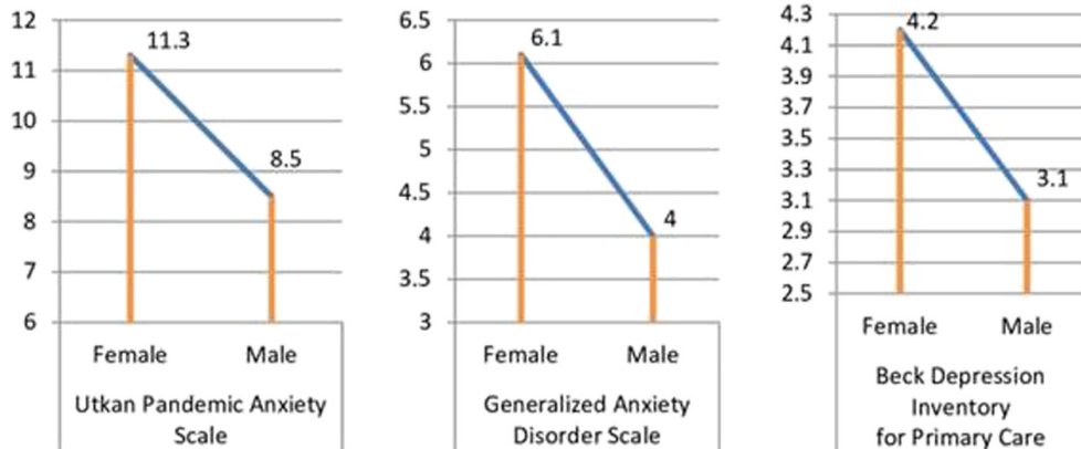
Figure 3. Comparison of the mean values of the scales in terms of gender, with Student's t-test ( n_{\text{female}} = 901 , n_{\text{male}} = 366 ).
