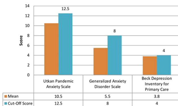
Figure 1. The mean and cut-off values of the scales.
