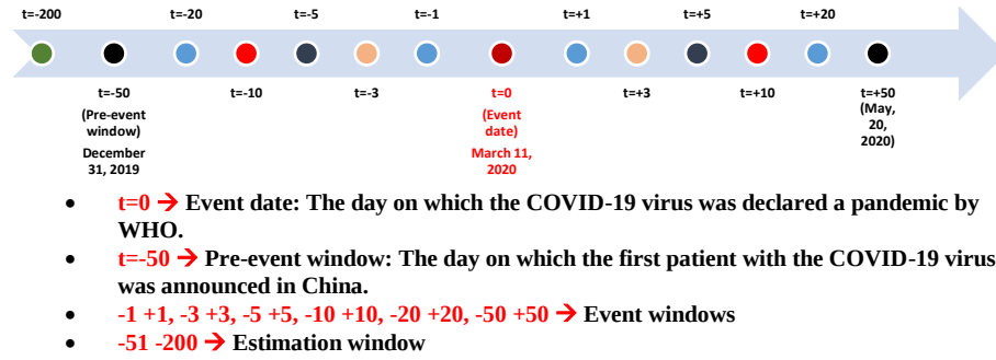
Figure 1. Event Date, Event Windows, Estimation Window
