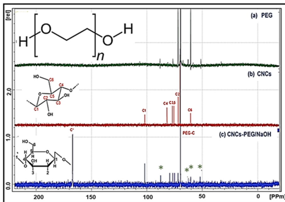
Fig. 3. ^{13}\text{C} NMR spectra of (a) PEG, (b) CNCs, (c) CNCs-PEG/NaOH solution.
