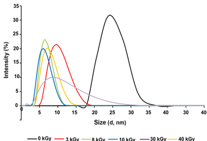
Fig. 5. DLS spectra of (CNCs-PEG/NaOH)/Gd 2 O 3 nanocomposite at different doses.
