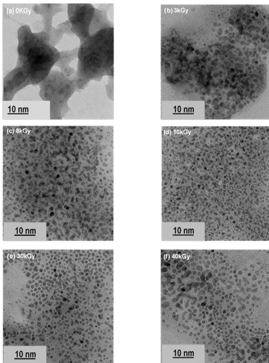
Fig. 4. TEM micrographs of nanocomposite at different doses (a) 0 kGy (b) 3 kGy, (c) 8 kGy, (d) 10 kGy, (e) 30 kGy and (f) 40 kGy.
