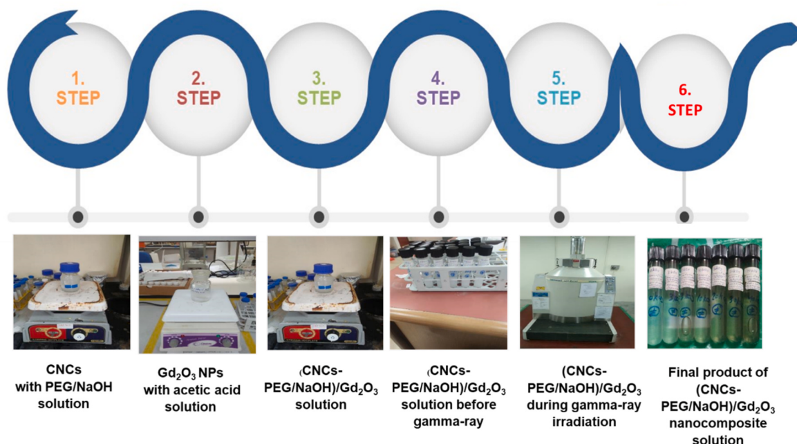
Fig. 1. Schematic representation of synthesized (CNC-PEG/NaOH)/Gd 2 O 3 through gamma-ray irradiation.
