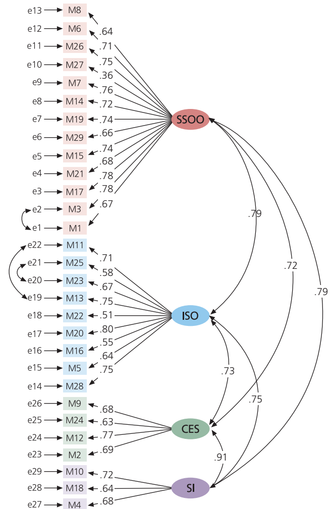
Figure 2. Path diagram.
