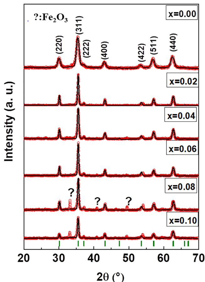
Fig. 1. XRD powder patterns of \text{Ni}_{0.4}\text{Cu}_{0.2}\text{Zn}_{0.4}\text{Tb}_x\text{Fe}_{2-x}\text{O}_4 ( x = 0.00-0.10 ) NSFs.
