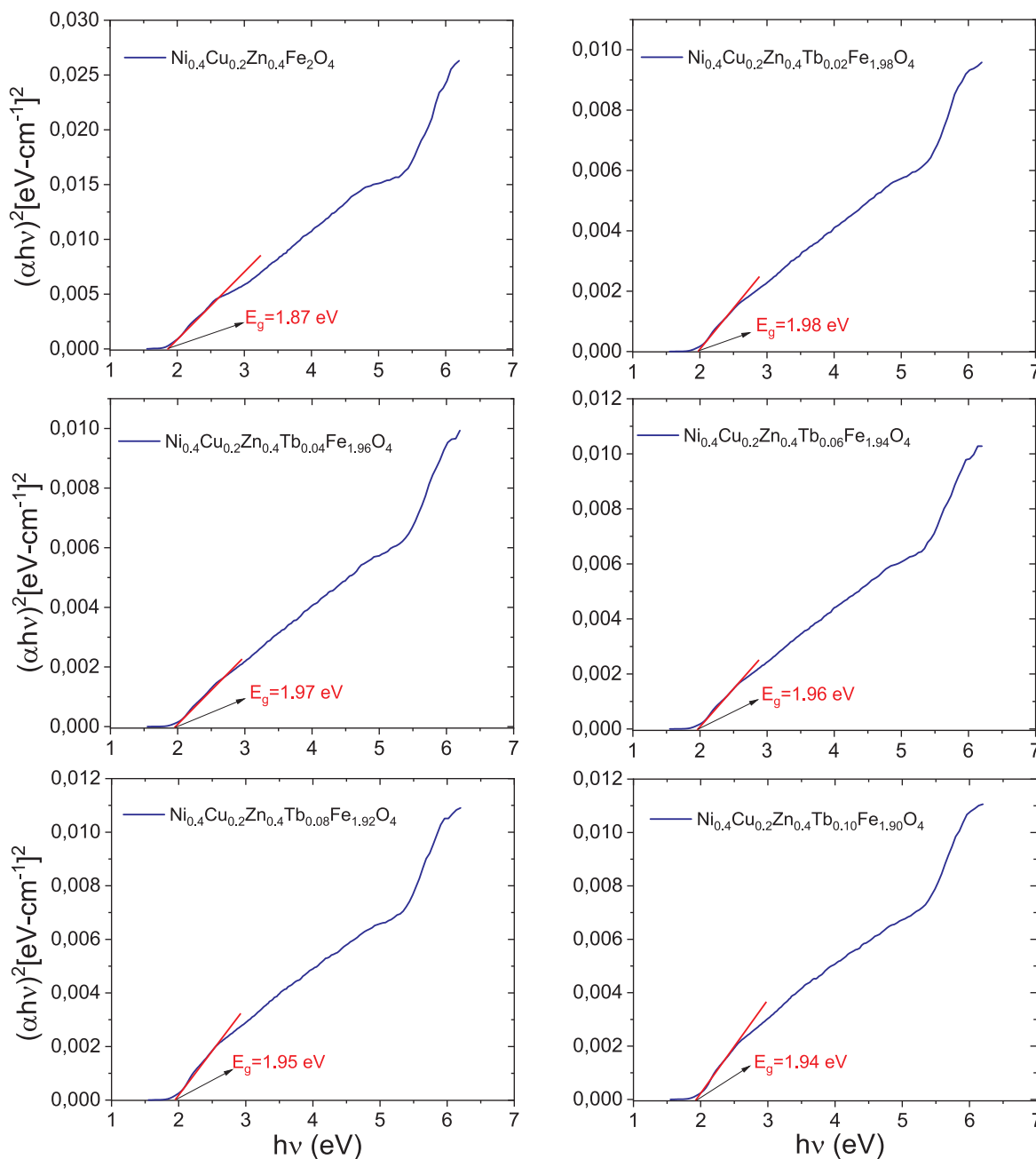
Fig. 8. Tauc plots of \text{Ni}_{0.4}\text{Cu}_{0.2}\text{Zn}_{0.4}\text{Tb}_x\text{Fe}_{2-x}\text{O}_4 ( x = 0.00\text{--}0.10 ) NSFs. Extrapolating the straight portion of graph to h\nu axis at the (\alpha h\nu)^2 = 0 determines the value of direct band gap.
