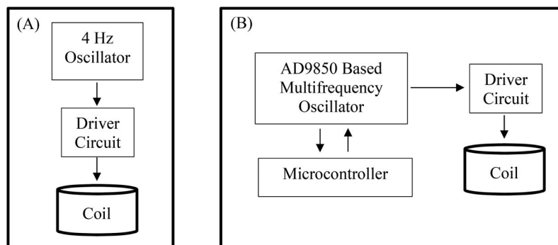
Figure 2. Block diagram of the control cards of PEMF devices used in this study. 4Hz single frequency(a), and AD9850 based multifrequency oscillator systems (B).
