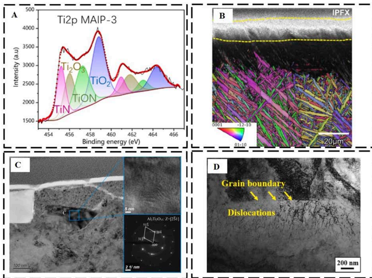
FIGURE 7 (A) XPS spectrum, (B) EBSD material grains, (C) TEM microstructure, (D) TEM dislocations and grain boundary. (A) Reproduced with permission (Zhang et al., 2022). Copyright 2022, Elsevier. (B) Reproduced with permission (Yu et al., 2024). Copyright 2024, Elsevier. (C) Reproduced with permission (Yang et al., 2024). Copyright 2024, Elsevier. (D) Reproduced with permission (Weng et al., 2022). Copyright 2022, Elsevier.
