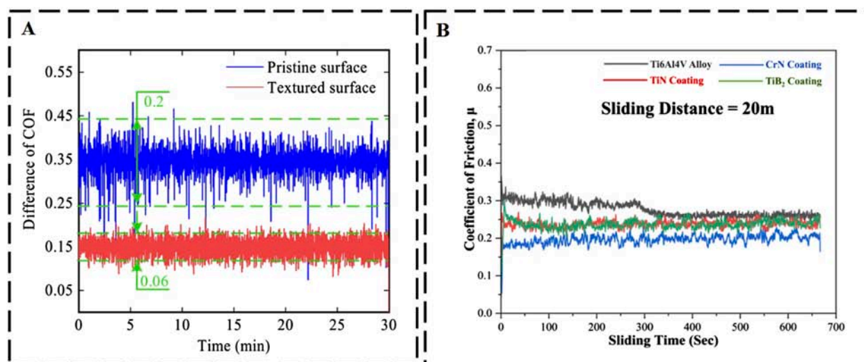
FIGURE 4 Force-time based friction graphs of Ti6Al4V alloy: (A) with laser texturing and simultaneous nitriding surface treatments, (B) with TiN, CrN and TiB 2 coating by RF magnetron sputtering deposition. (A) Reproduced with permission (Wang et al., 2023a). Copyright 2023, Elsevier. (B) Reproduced with permission (Narayana and Saleem, 2024). Copyright 2024, Elsevier.
