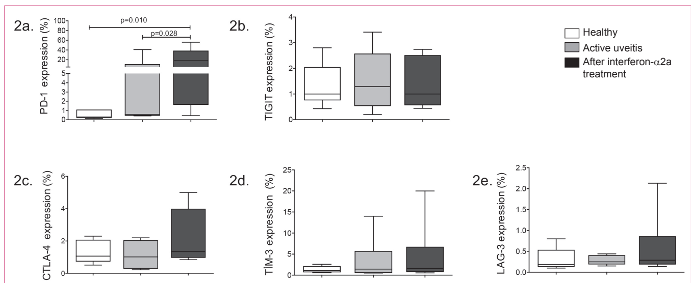
Figure 2 a-e. Immune checkpoint receptor expressions in the monocytes of the patients and control subjects. Immune checkpoint receptor expressions of CD14 expressing monocytes were shown in healthy controls, patients with active uveitis and patients treated with interferon \alpha -2a (a-e). Bar graphs represent median and interquartile range.
