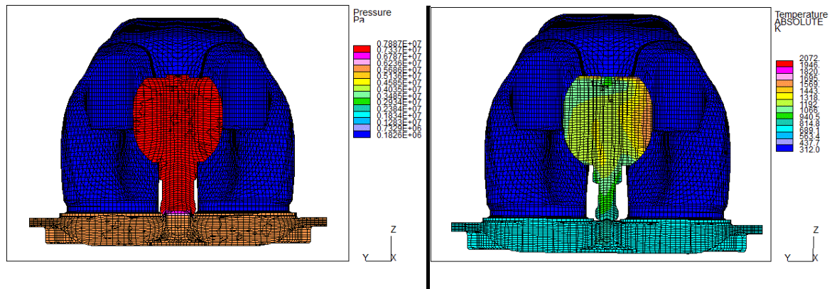
Figure 9. Pressure and temperature contours near TDC.
