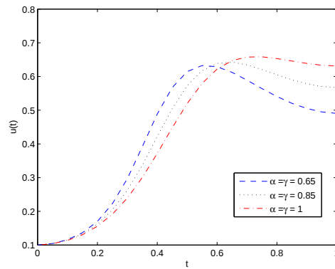
FIGURE 3. Resulting graph of u(t) for different \alpha = \gamma values, N = 20 .
