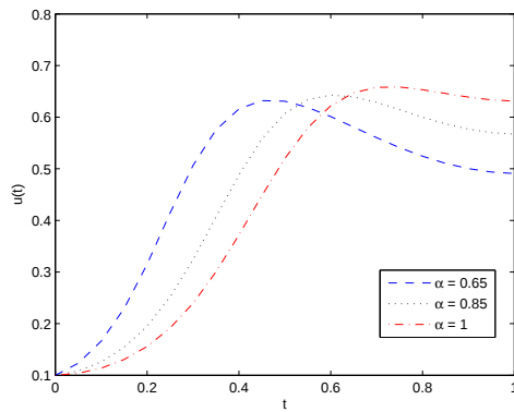
FIGURE 2. Resulting graph of u(t) for different \alpha values, N = 20 .
