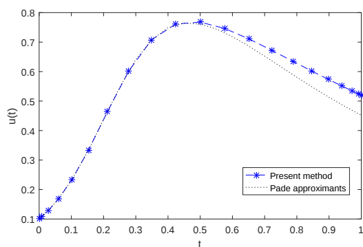
FIGURE 1. A comparison when N = 20 , \alpha = 1 , K = 0.1 .
