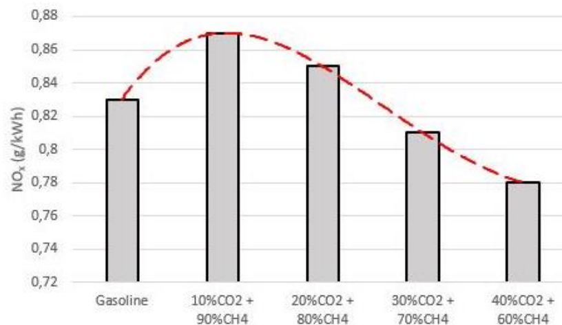
Figure 6. Effect of different level of CO 2 and CH 4 addition on specific NO x emissions
