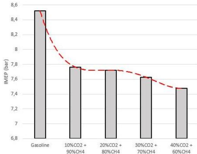
Figure 3. Effect of using CH 4 at different CO 2 levels on indicated mean effective pressure
