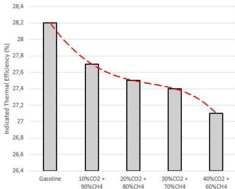
Figure 2. Effect of different level of CO 2 and CH 4 addition on indicated thermal efficiency
