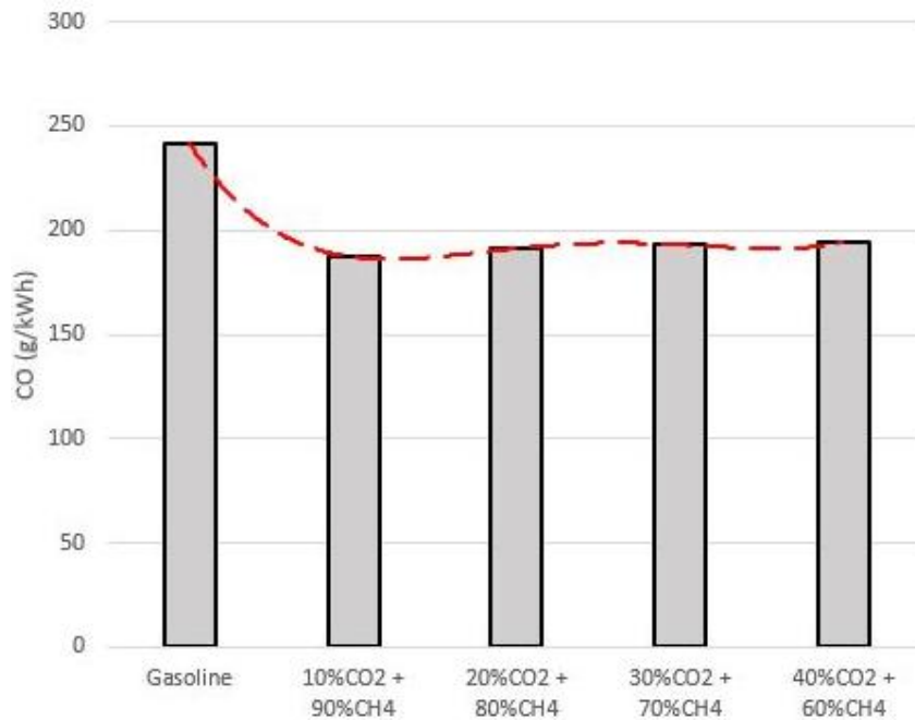
Figure 4. Effect of different level of CO 2 and CH 4 addition on specific CO emissions
