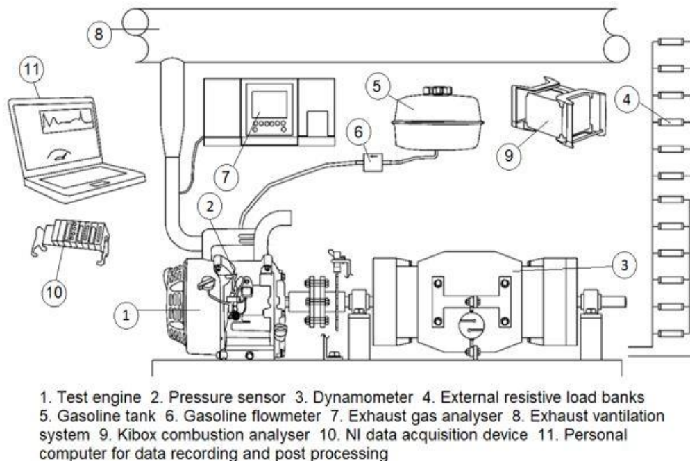
Figure 1. Schematic diagram of engine test system
