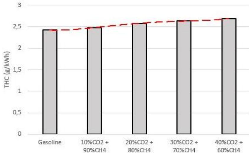
Figure 5. Effect of different level of CO 2 and CH 4 addition on specific THC emissions
