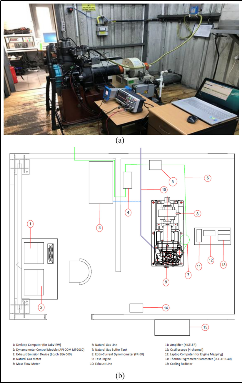
Figure 1. (a) Picture of testing set and (b) schematic view of testing set.
