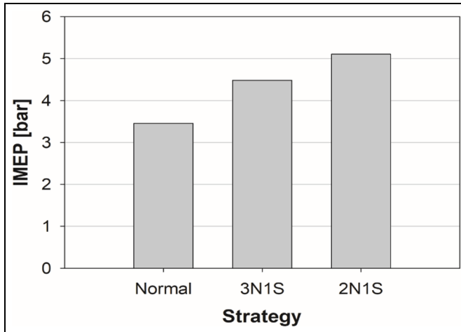
Figure 4. The comparison of indicated mean effective pressure.
