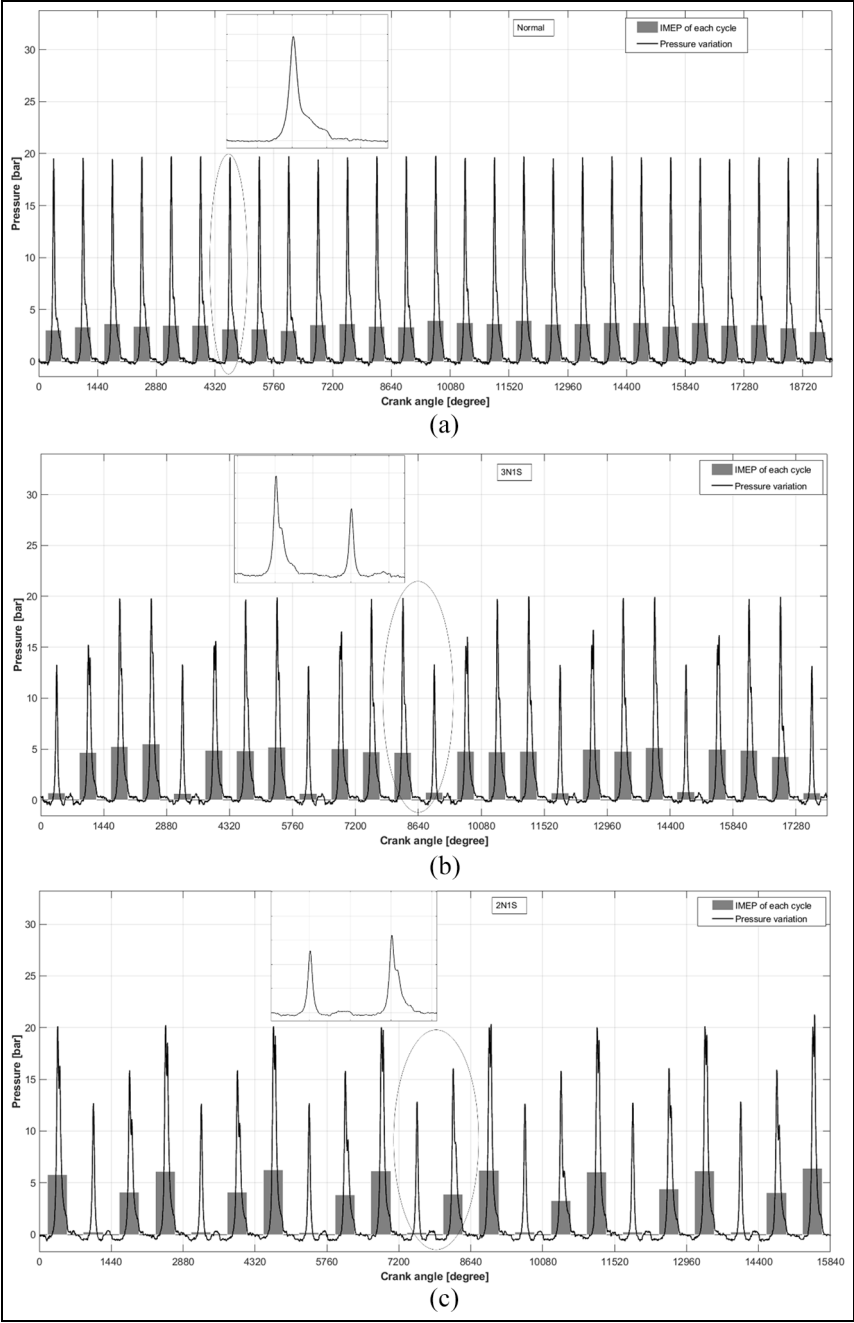
Figure 9. (a) In-cylinder pressure at normal engine operation, (b) in-cylinder pressure at 3N1S engine operation, and (c) in-cylinder pressure at 2N1S engine operation.
