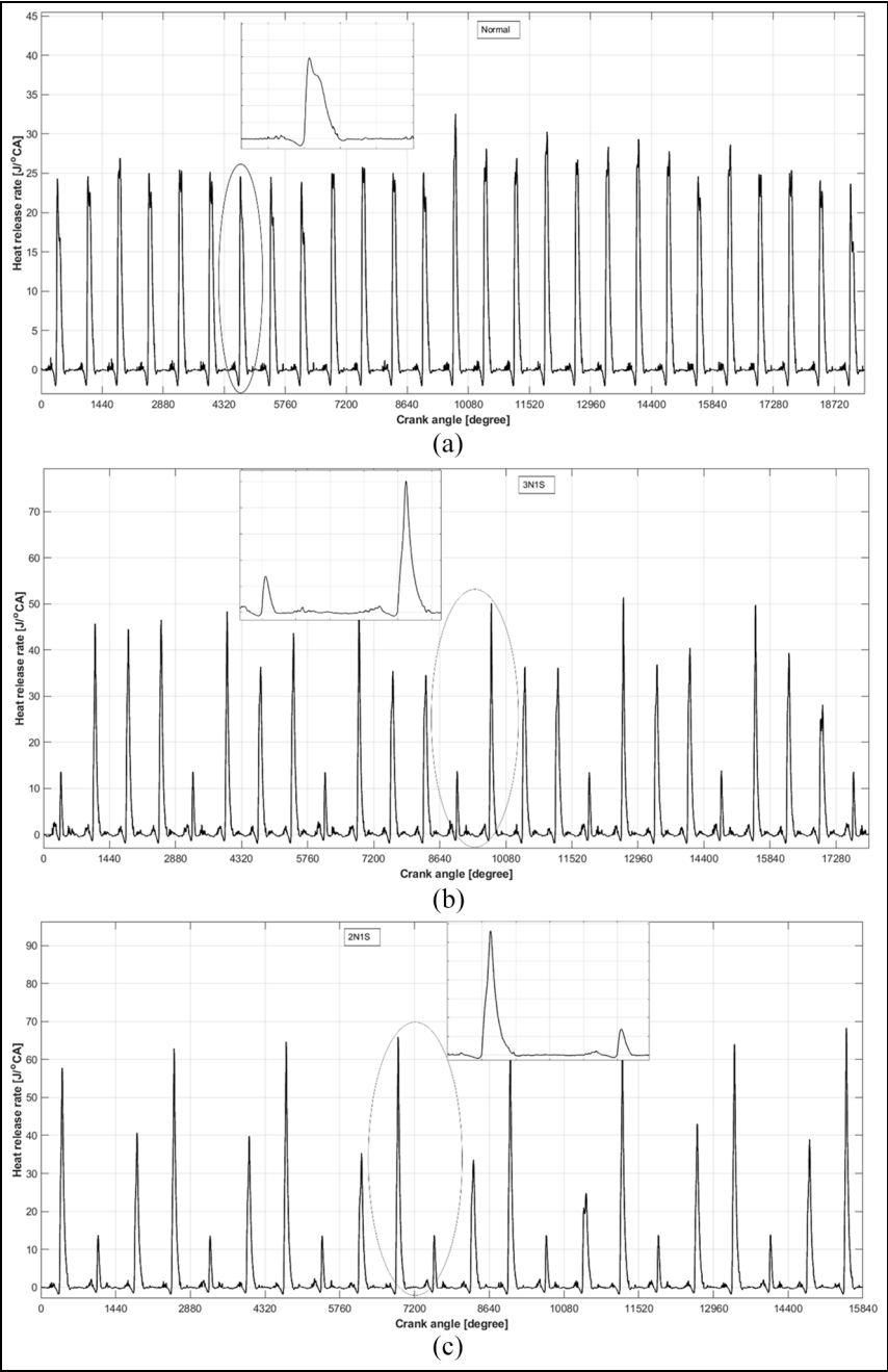
Figure 10. (a) Heat release rate at normal engine operation, (b) heat release rate at 3NIS engine operation, and (c) heat release rate at 2NIS engine operation.
