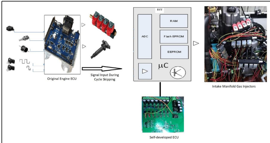
Figure 3. Schematic view of the self-developed electronic control unit.
