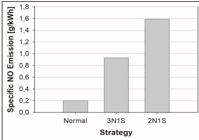
Figure 8. The comparison of NO x emission values.
