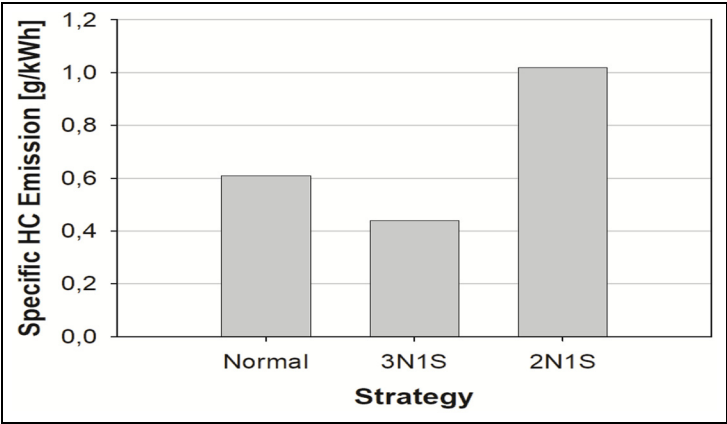
Figure 7. The comparison of HC emission values.
