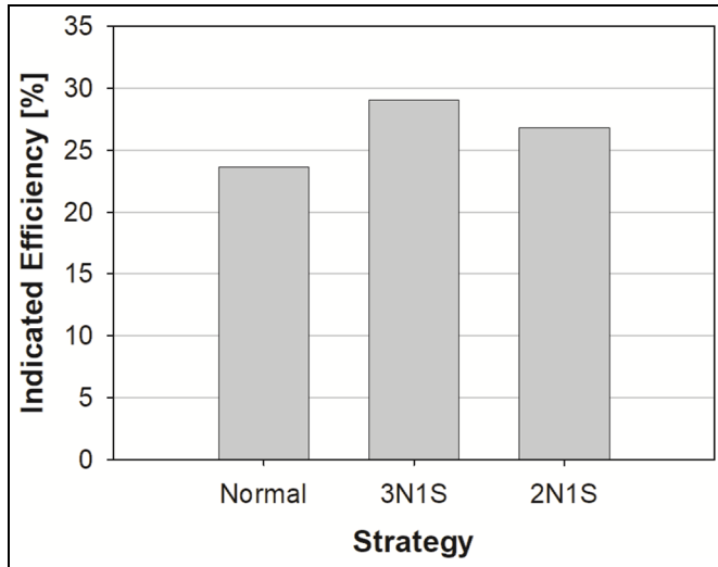
Figure 5. The comparison of indicated efficiency.
