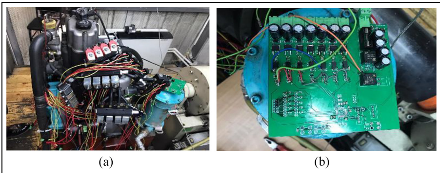
Figure 2. View of (a) gas injectors have placed in intake manifold and (b) the electronic control unit.
