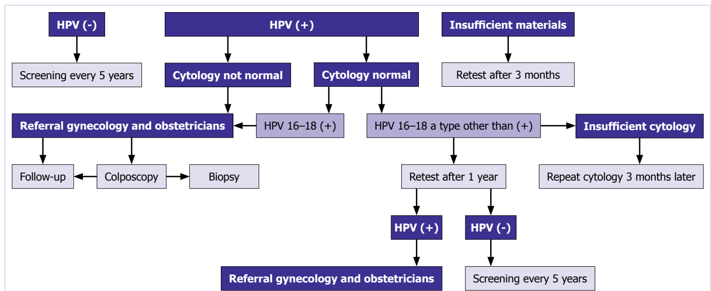
FIGURE 1. HPV algorithm.
