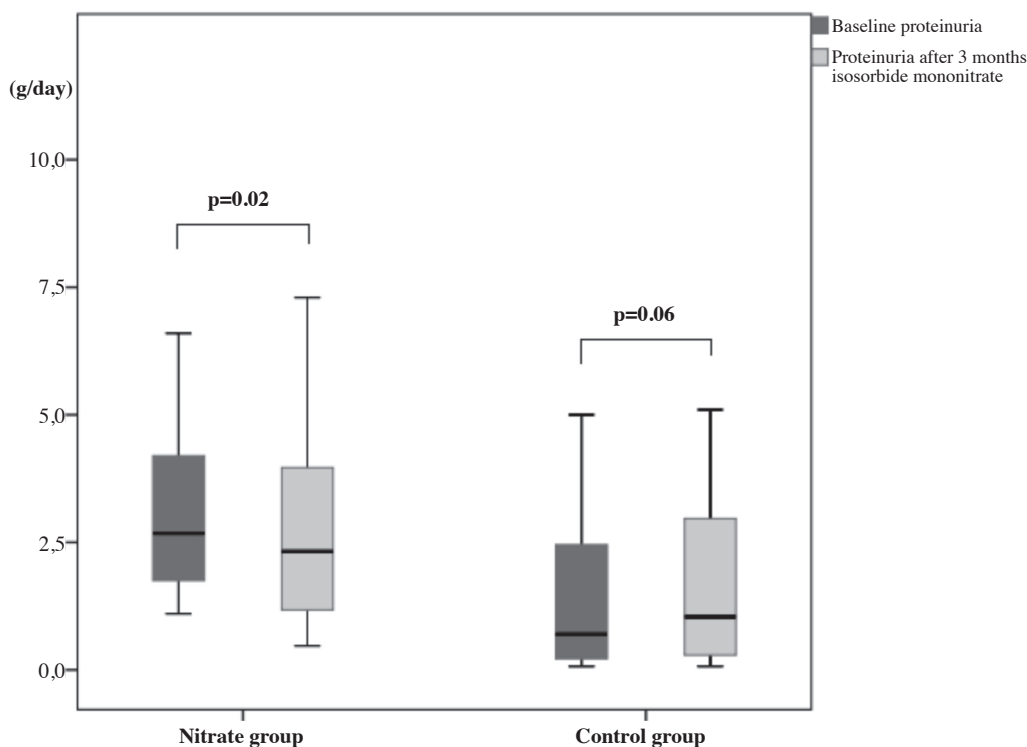
Figure 1. Univariate analysis.
