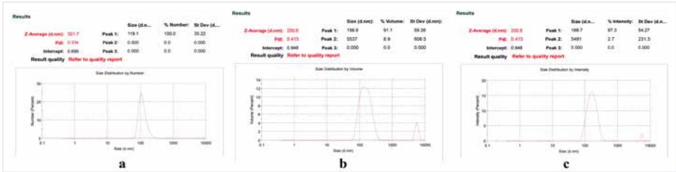
Figure 2. Particle size distribution of the optimized formulation; 50mg CLX in 50mgPLGA/20mL
