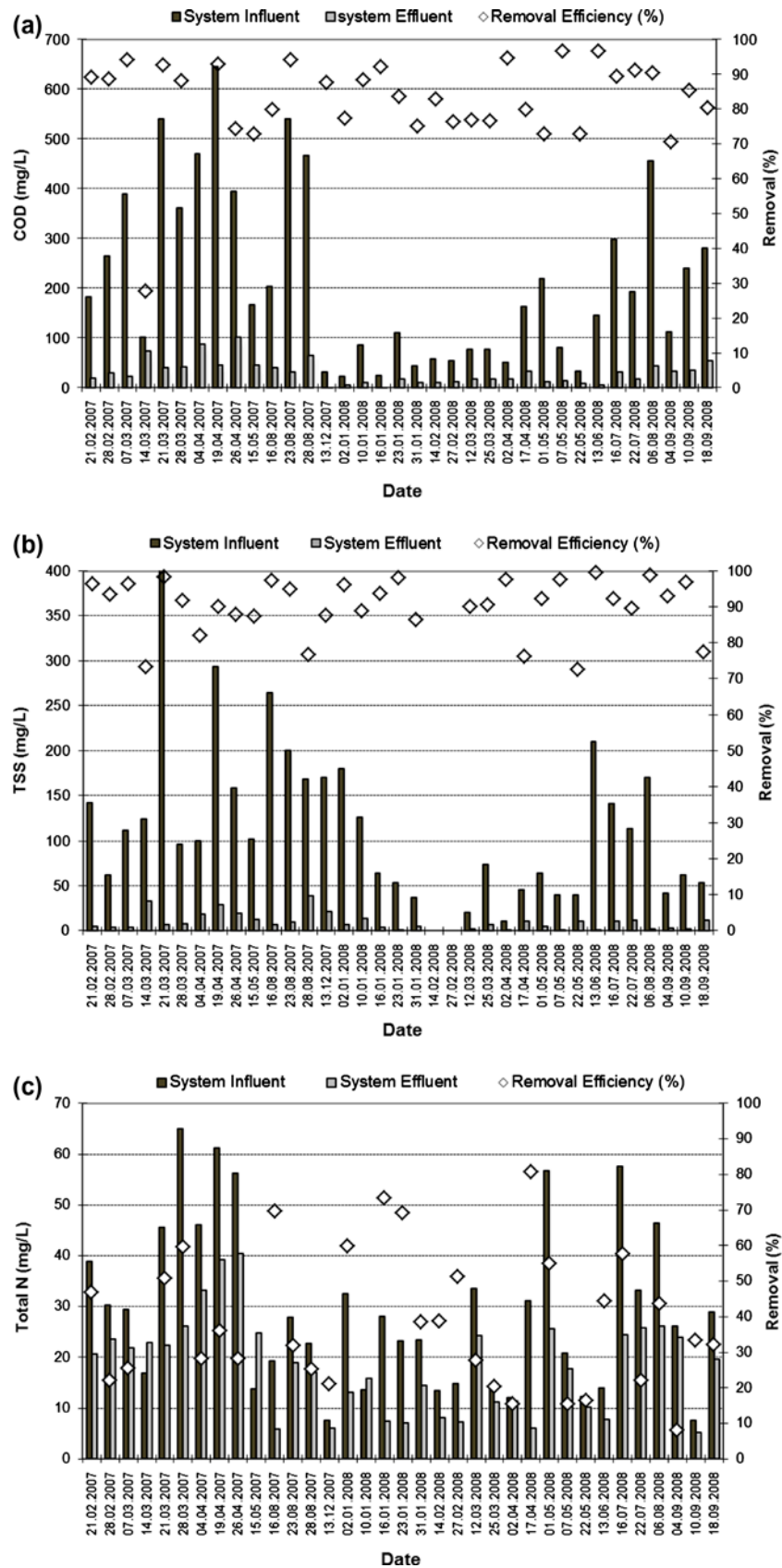
Fig. 5. Performance of the treatment system in Orucoglu village in terms of (a) COD, (b) TSS, and (c) TN.
