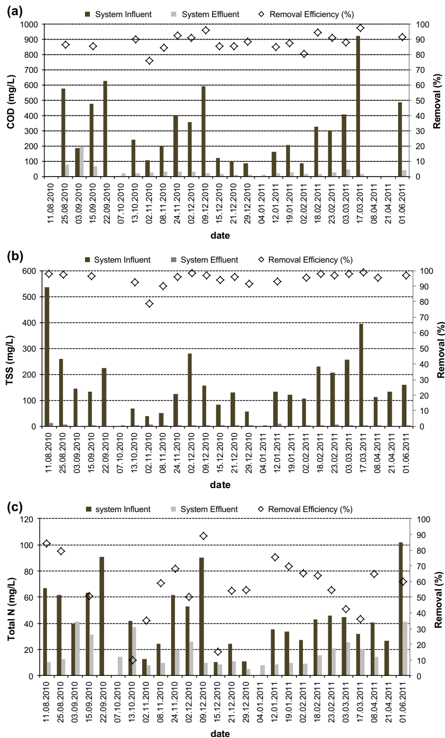
Fig. 3. Performance of the treatment system in Balcik village in terms of (a) COD, (b) TSS, and (c) TN.
