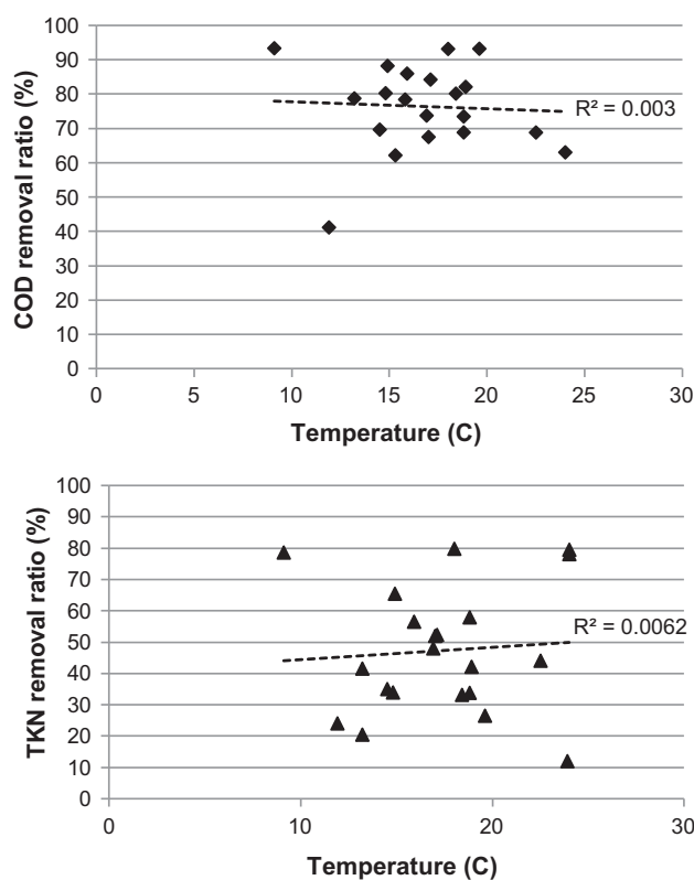
Fig. 4. Linear regression of COD and TKN removal efficiencies with respect to temperature in the CW system in Balcik.
