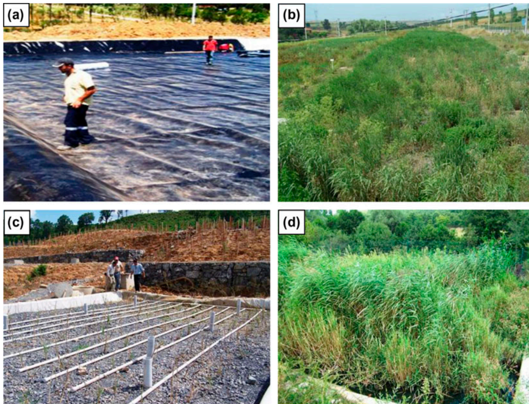
Fig. 1. Photographs from construction and operation of wetland systems in Balcik (a, b) and Orucoglu (c, d).
