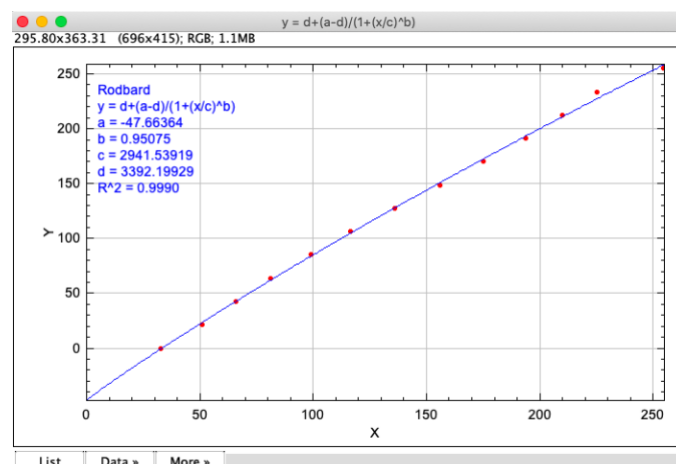
Figure 3. Calibration curve
