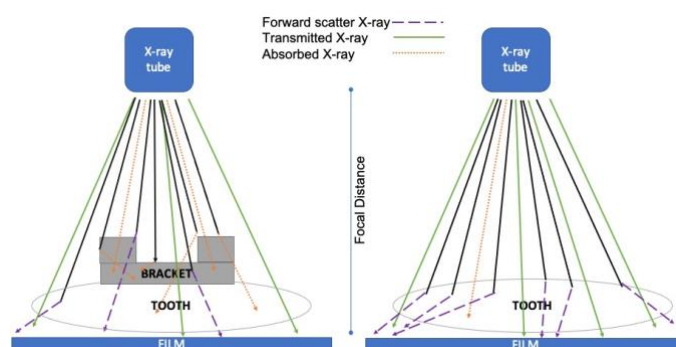
Figure 4. Scattering types
