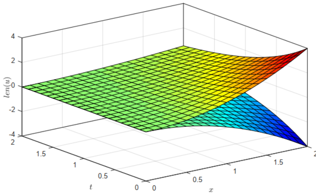
FIGURE 5. The approximate solution of Ex. 2 for (ii)-differentiability.
