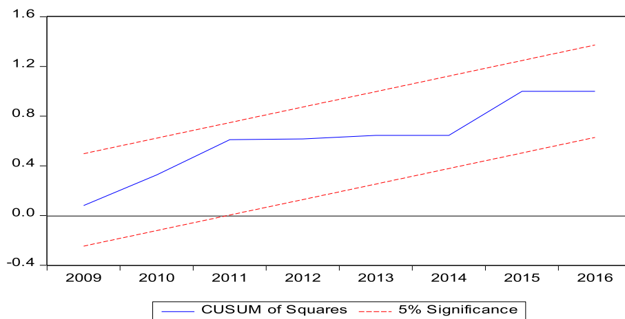
Fig. 5. CUSUMSQ.
