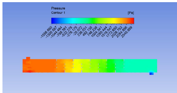
Figure 8. Pressure distribution of conventional one-piece baffle plate type heat exchanger: gap = 75 mm; mass flow rate = 1.2 kg/s.
