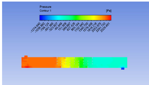
Figure 7. Pressure distribution of conventional one-piece baffle plate type heat exchanger: gap = 50 mm; mass flow rate = 1.2 kg/s.
