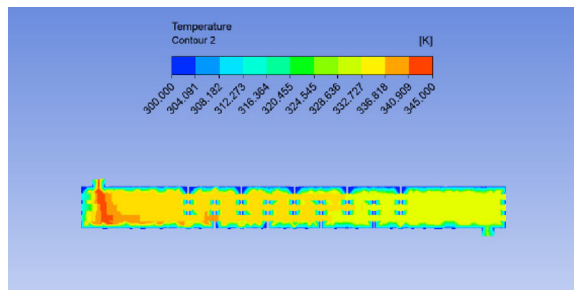
Figure 9. Temperature distribution of conventional one-piece baffle plate type heat exchanger: gap = 75 mm; mass flow rate = 1.2 kg/s.
