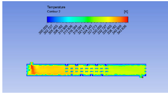
Figure 6. Temperature distribution of conventional one-piece baffle plate type heat exchanger: gap = 50 mm; mass flow rate = 1.2 kg/s.
