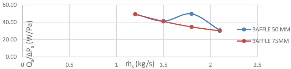
Figure 24. Relationship between heat transfer rate per pressure drop and mass flow rate.
