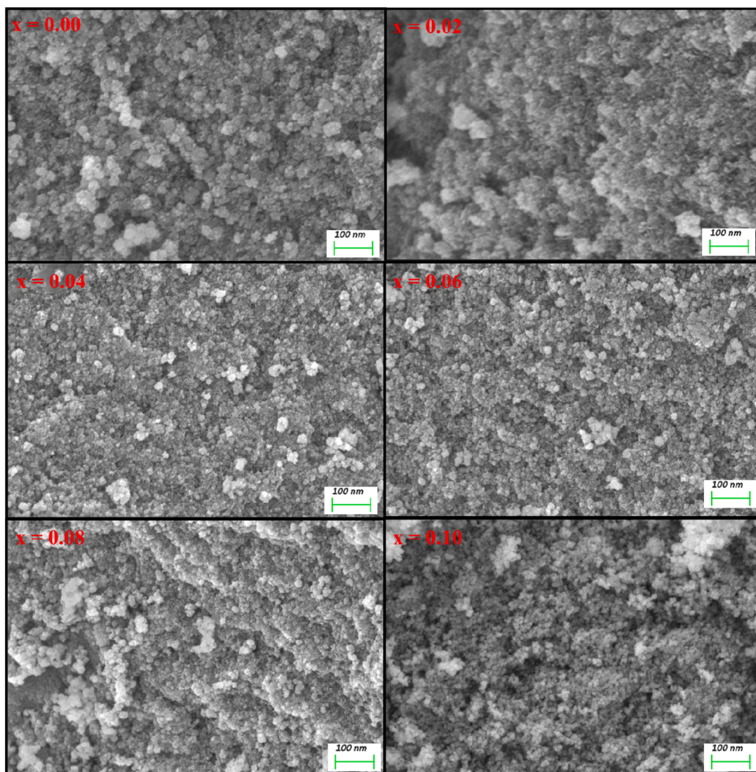
Figure 3. FE-SEM images of \text{Co}_{0.3}\text{Ni}_{0.5}\text{Mn}_{0.2}\text{Eu}_x\text{Fe}_{2-x}\text{O}_4 ( 0.00 \leq x \leq 0.10 ) nanospinel ferrites.
