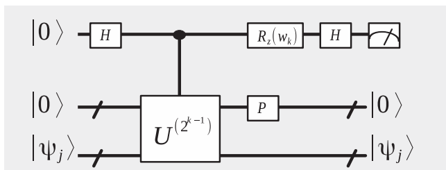
Fig. 1. The k th iteration of the phase estimation algorithm: In the circuit, |\psi_j\rangle is an approximate eigenvector of \mathcal{H} and w_k = -2\pi(0.0\phi_k\phi_{k-1} \dots \phi_a) , where \phi_k, \phi_{k-1}, \dots, \phi_a represents the previously measured bit values.
