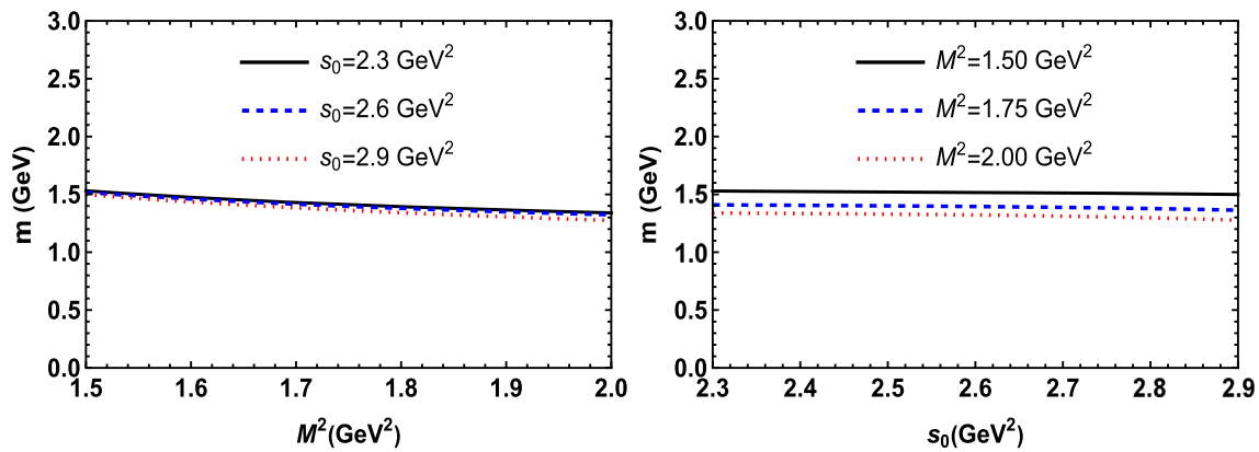
Fig. 2 Left: The dependence of the mass on the Borel parameter M^2 at different values of the threshold parameter s_0 . Right: The dependence of the mass on the threshold parameter s_0 at different values of the Borel parameter M^2
