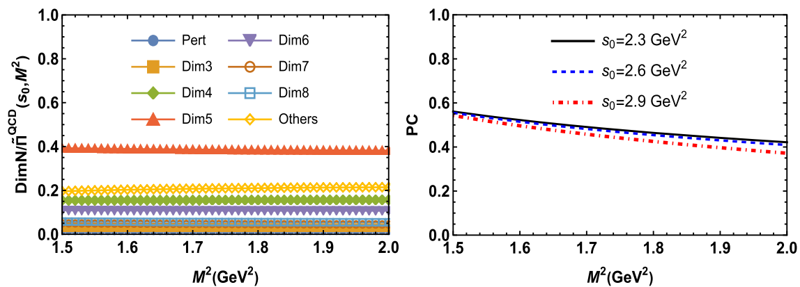
Fig. 1 Left: Contributions of different dimensions in the QCD side's result as a ratio of the contribution of each dimension to the total QCD result at the central value of s_0 . Right: The pole contribution for different values of s_0
