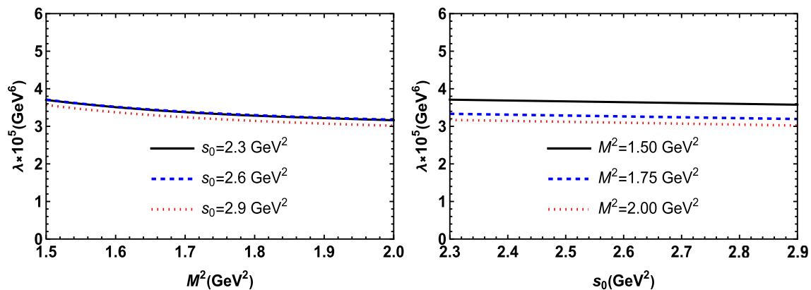
Fig. 3 Left: The dependence of the current coupling constant on the Borel parameter M^2 at different values of the threshold parameter s_0 . Right: The dependence of the current coupling constant on the threshold parameter s_0 at different values of the Borel parameter M^2
