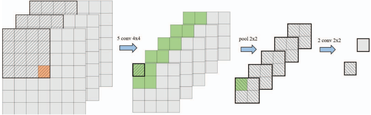
Fig 4. Representation of convolutional network structure
