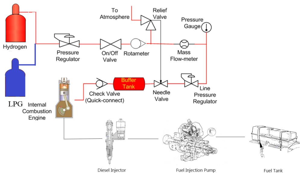
Figure 2. LPG + H 2 and diesel fuel system
