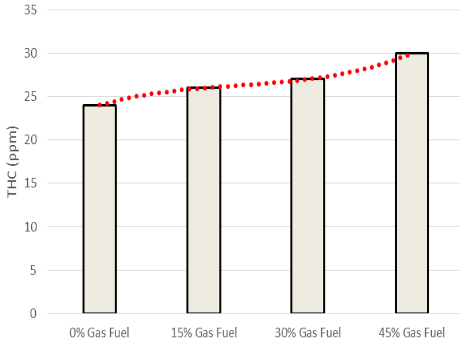
Figure 5. Effect of various level of LPG+H 2 addition on THC emissions
