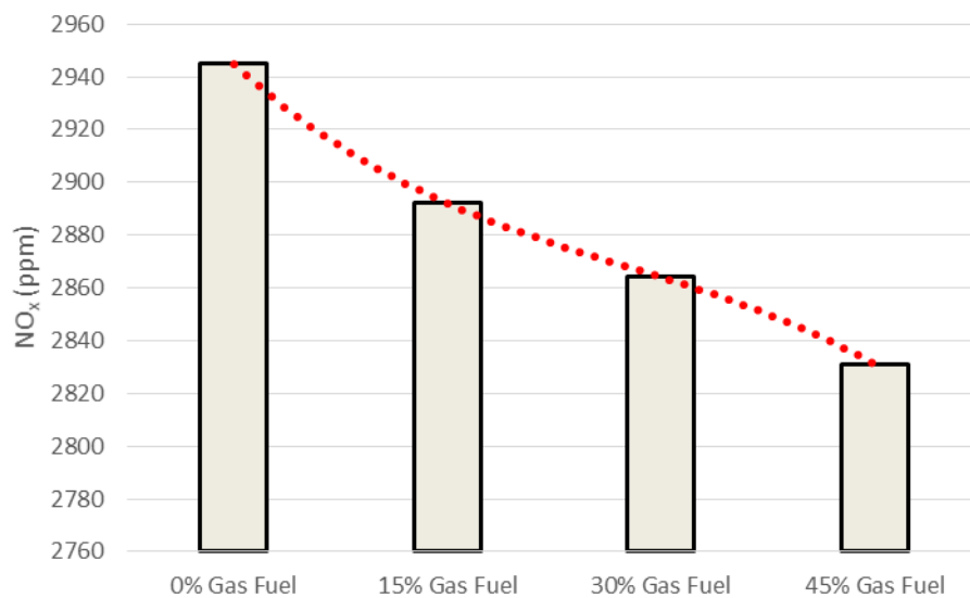
Figure 6. Effect of various level of LPG+H 2 addition on NO x emission
