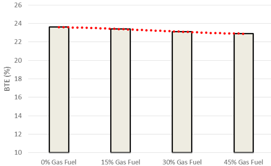
Figure 3. Effect of various level of LPG+H 2 addition on brake thermal efficiency
