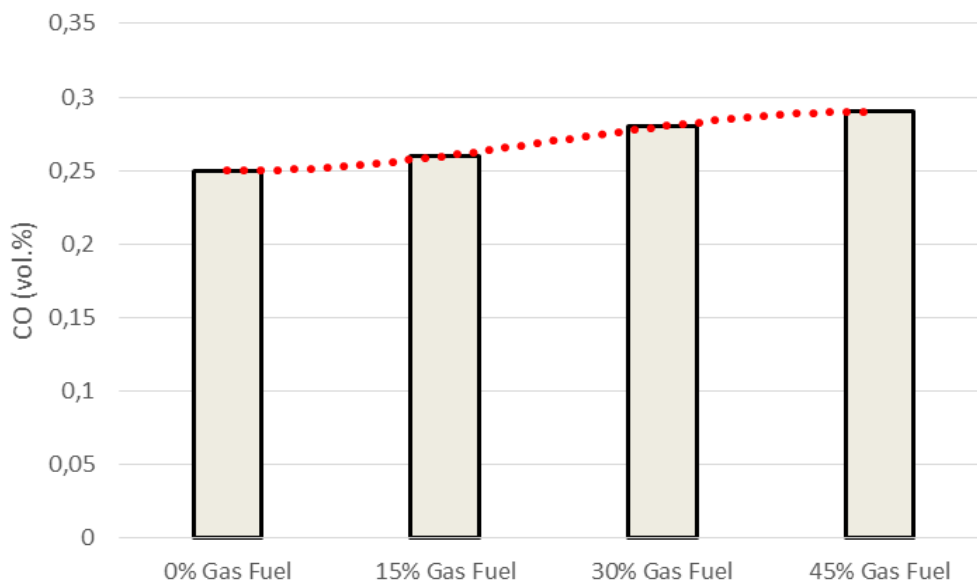
Figure 4. Effect of various level of LPG+H 2 addition on CO emissions
