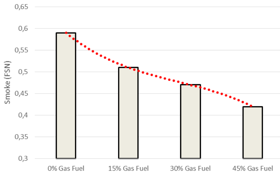
Figure 7. Effect of various level of LPG+H 2 hydrogen addition on smoke emission
