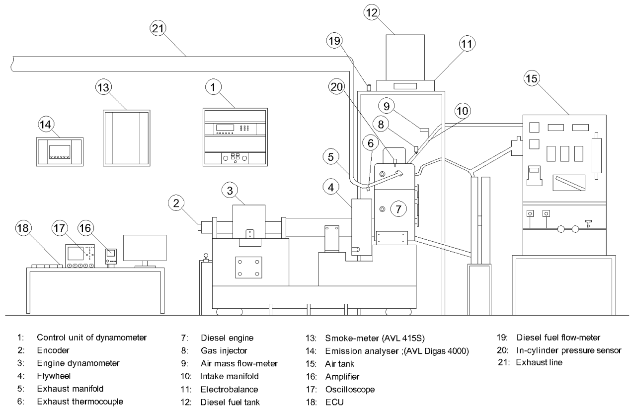
Figure 1. Test setup schematics
