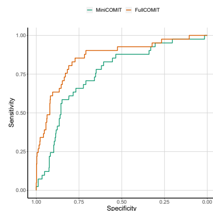
FIGURE 1 ROC curves
