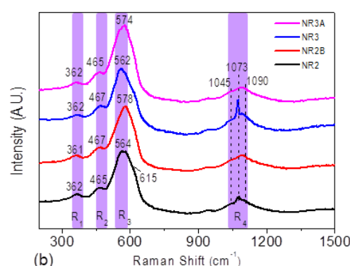
Figure 2. (a) FTIR and (b) Raman spectrum of NR2, NR2B, NR3, and NR3A.
