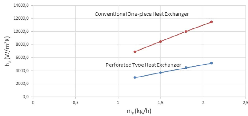
Figure 20. Results of variation of heat transfer coefficient with mass flow rate.
