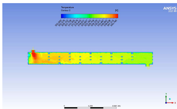
Figure 17. Temperature distribution of conventional type baffle plate heat exchanger at mass flow rate = 1.2.
