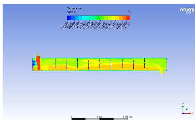
Figure 16. Temperature distribution of perforated type baffle plate heat exchanger at mass flow rate = 1.2.
