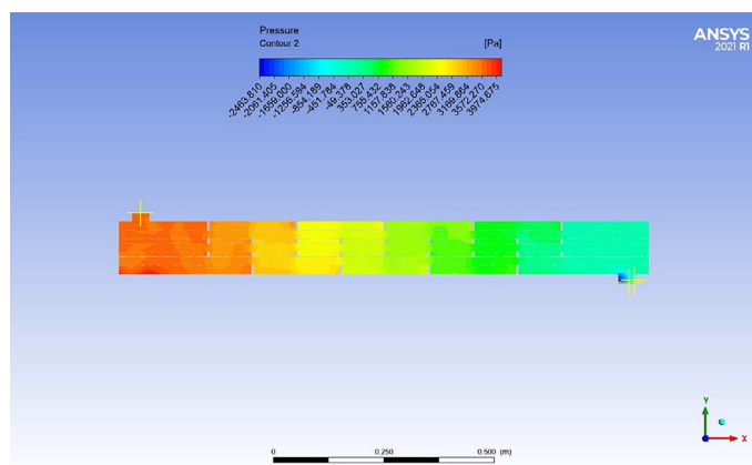
Figure 15. Pressure distribution of conventional type baffle plate heat exchanger at mass flow rate = 1.5.
