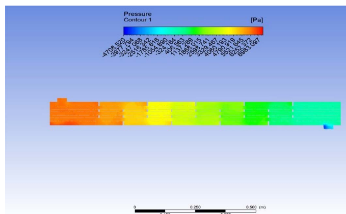
Figure 6. Pressure distribution of conventional type baffle plate heat exchanger at maximum mass flow rate = 2.1.
