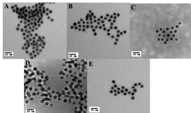
Fig. 2 TEM images of different nanoparticles: (A) commercial AuNPs, (B) AuNP-MHDA, (C) AuNP-peptide stained by phosphotungstic acid, and (D) Au-peptide-IgY stained by phosphotungstic acid. (E) Control particles: commercial AuNPs stained by phosphotungstic acid.
