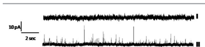
Fig. 9 Current-time recordings for a 28 nm-diameter pipette in a 15 mM NaCl + 10 mM PB (pH 7) solution containing (I) 0 and (II) 1 nM of Au-peptide-IgY particles. V = -200 mV. i_0 = -655 pA (I) and -545 pA (II).
