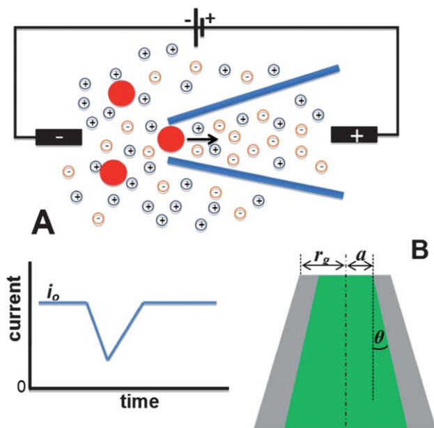
Fig. 1 (A) Simplified schematic representation of resistive-pulse sensing with a nanopipette. In the presence of nanoparticles, blockage events can be seen in the current vs. time curve. (B) Parameters defining the nanopipette geometry.
