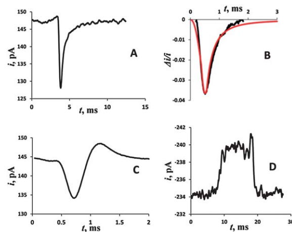
Fig. 10 Current pulses obtained in solutions containing (A and C) AuNP-peptide, (B) Au-MHDA, and (D) AuNP-peptide-IgY. (B) Experimental (black) and theoretical (red) current-time pulses for the translocation of a Au-MHDA through a 34 nm-diameter pipette.
