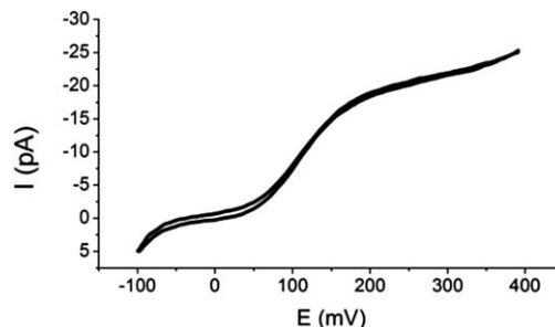
Fig. 4 Steady-state voltammogram of \text{ClO}_4^- transfer across the DCE–water interface obtained with a 25 nm-radius pipette in cell 1 with the potential sweep rate of 50 \text{ mV s}^{-1} .
