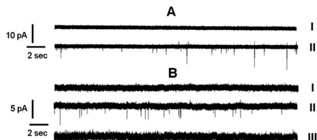
Fig. 7 Current-time recordings obtained with a (A) 28 nm-diameter and (B) 32 nm-diameter pipette in a 15 mM NaCl + 10 mM PB (pH 7). (A) Solution contained: 0 (trace I) and 2 nM (trace II) of 10 nm-diameter AuNP; V = 150 mV. i_0 = 156 pA (I) and 134 pA (II). (B) Solution contained: 0 (I) and 1.8 nM (II, III) of AuNP-peptide. V = 100 mV (I, II) and -100 mV (III). i_0 = 222 pA (I), 233 pA (II) and -363 pA (III).
