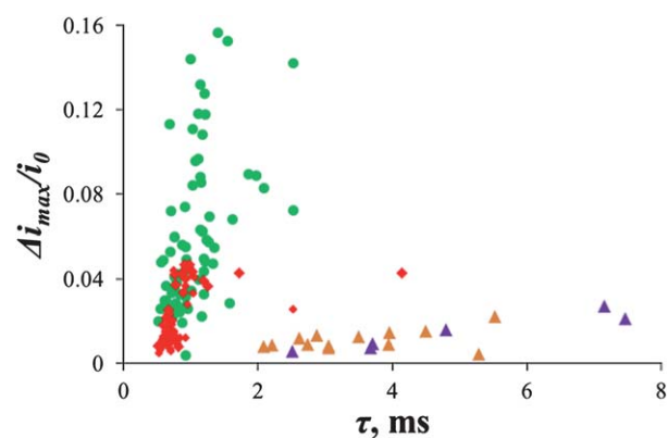
Fig. 8 Scatter plots of the normalized maximum current change versus peak width for AuNP–peptide translocation experiments with three different pipettes. Pipette diameter (nm): 108 (triangles) 28 (diamonds), and 22 (circles). The applied voltage (mV) was: 200 (green; total recording time 24.3 min), 300 (red; 40 s), 800 (purple; 8 min) and 900 (orange; 15.3 min). For other parameters, see Fig. 7.
