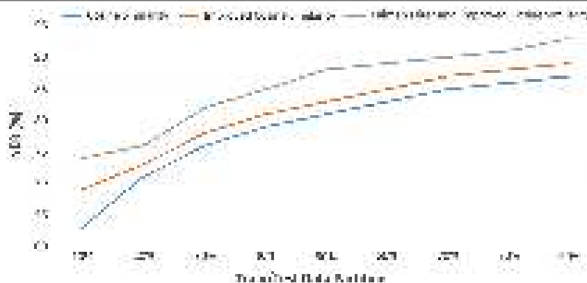
Fig. 8. Accuracy results with cosine similarity, improved cosine similarity, and Kalman filter-improved cosine similarity.
