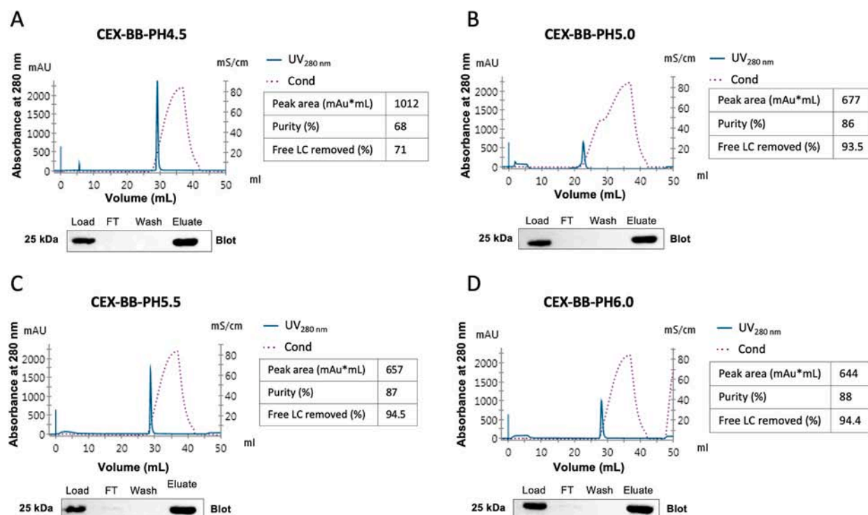
Fig. 2. Selecting optimal binding conditions for the Fab in cation-exchange chromatography (CEX). Chromatograms of CEX runs on a HiTrap SP-FF column using 1 mL eluate obtained from Protein L step. Binding with A) pH 4.5 B) pH 5.0 C) pH 5.5 D) pH 6.0 with a linear gradient to 100 % Buffer B over 10 CV. Immunoblots of peaks and purity ratios obtained by CE-SDS were given. Full, non-adjusted blots are represented in Supplementary File Fig. 2.
