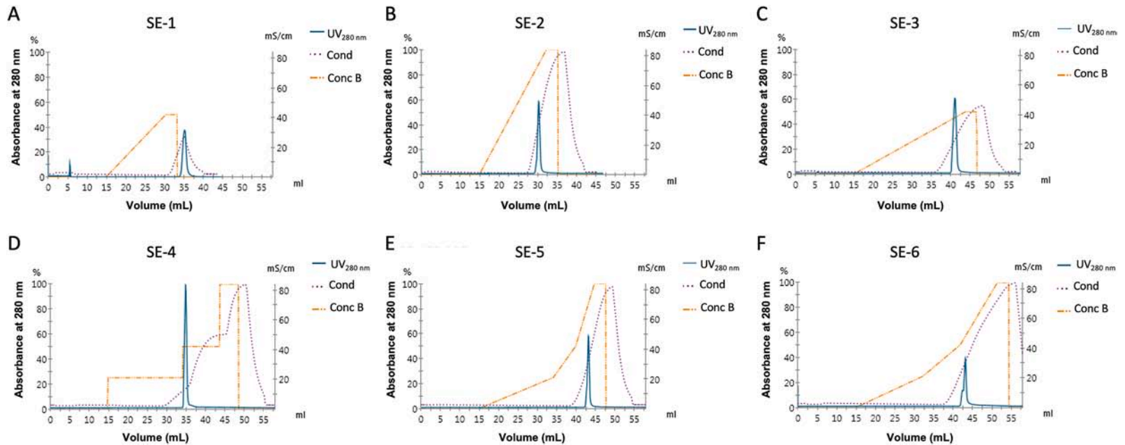
Fig. 3. Salt elution profiles of ion-exchange chromatography using SP-FF column with different elution conditions at a flow rate of 0.6 mL/min. A) 50 % concentration B with linear gradient over 16 C V B) 100 % concentration B with linear gradient over 18 C V C) 50 % concentration B with linear gradient over 30 C V D) 25 %, 50 % and 100 % concentration B with step gradient over 18, 10 and 10 C V, respectively E) 25 %, 50 % and 100 % concentration B with linear gradient over 20, 6 and 5 C V, respectively F) 25 %, 50 % and 100 % concentration B with linear gradient over 20, 10 and 5 CV, respectively. SE: Salt elution, Cond: Conductivity, Conc B: Concentration B (20 mM sodium phosphate, 1 M NaCl pH 6.0).
