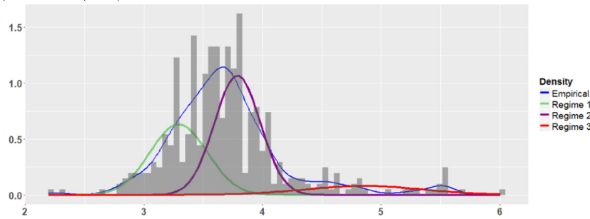
Fig. 2. Probability densities for the three-regime HSSM. A) Queensland (QLD). B) New South Wales (NSW). C) Victoria (VIC). D) South Australia (SA). E) Tasmania (TAS). (For interpretation of the references to color in this figure, the reader is referred to the web version of this article.)
