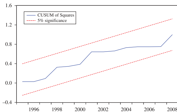
Figure 3. CUSUM of squares of the NARDL model.
