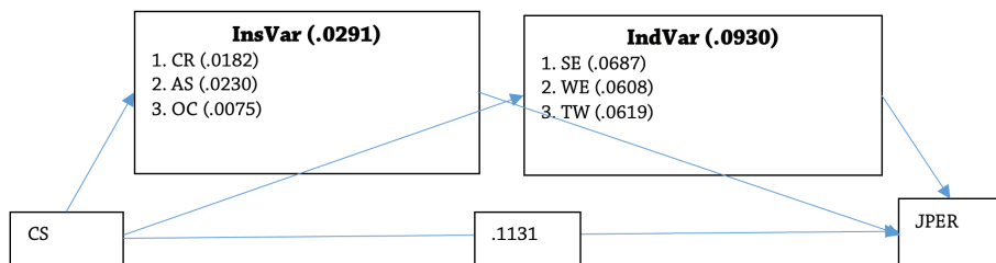
Figure 12. The effect rates of the mediating variables over the effect of CS on JPER
