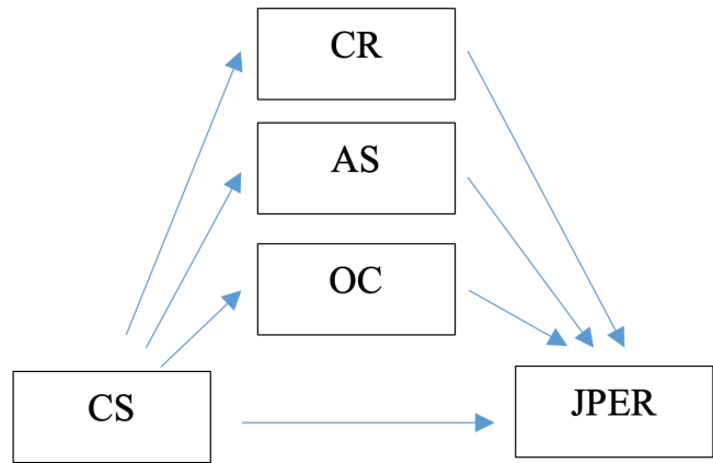
Figure 5. The model for H 5
