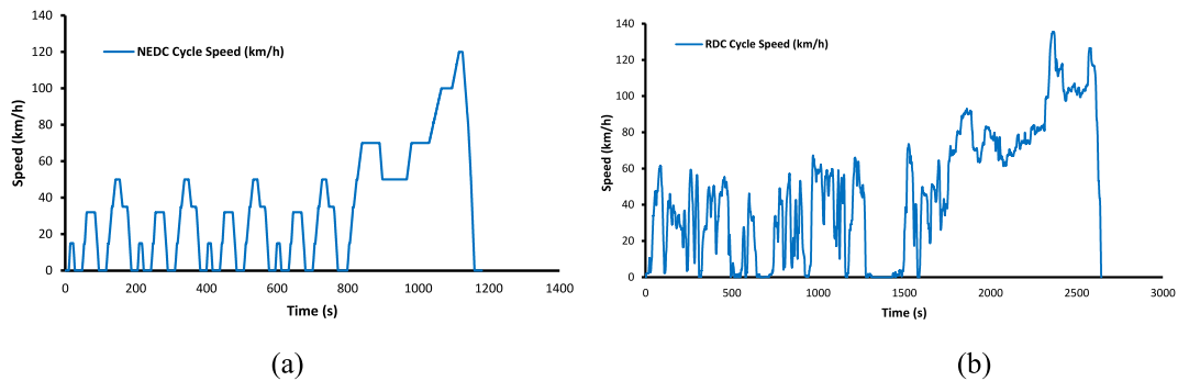
Fig. 4. Cycle profile for (a) NEDC (b) RDC.
