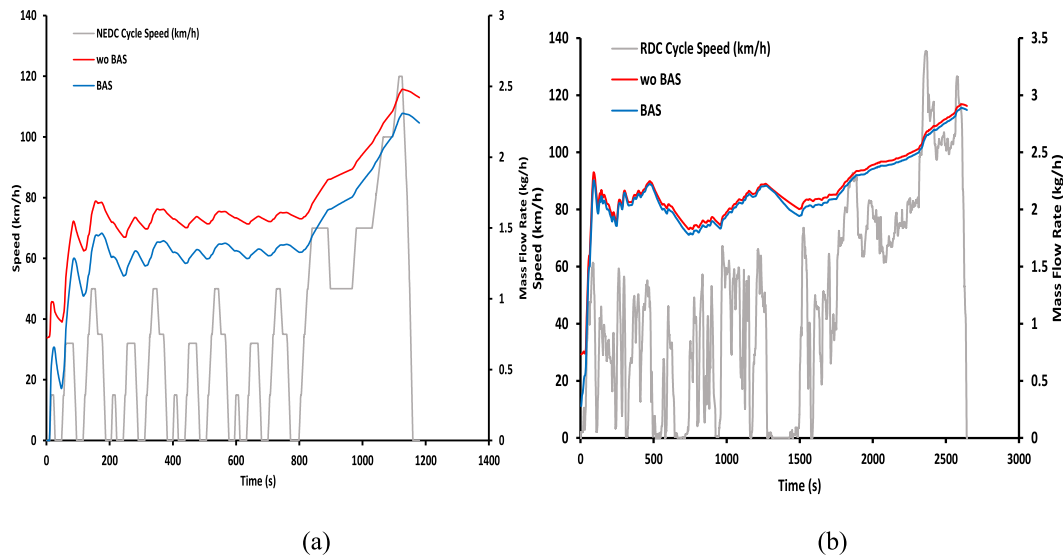
Fig. 5. Fuel flow rate with vs without BAS (a) NEDC (b) RDC.
