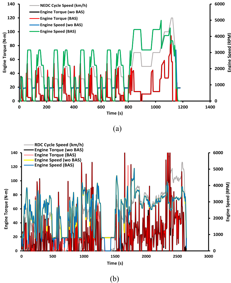
Fig. 6. Engine Speed and Torque with vs without BAS (a) NEDC (b) RDC.
