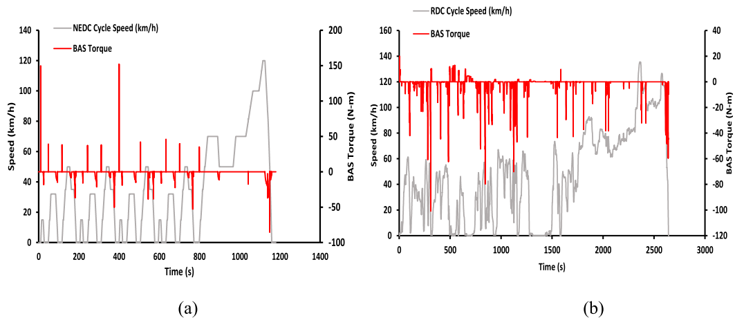
Fig. 8. BAS torque (a) NEDC and (b) RDC
