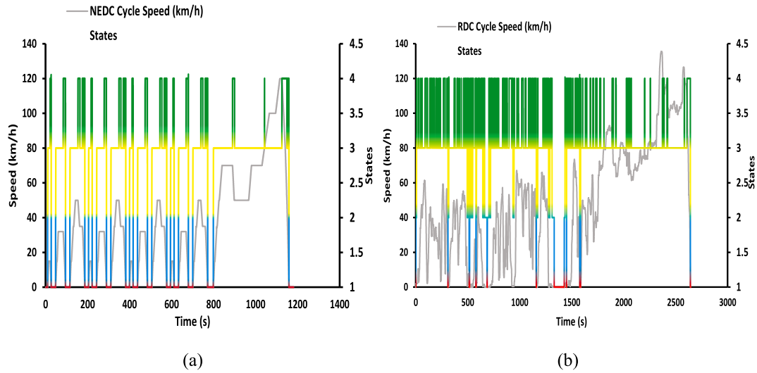
Fig. 7. BAS states (a) NEDC and (b) RDC
