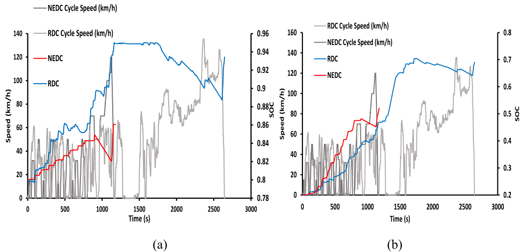
Fig. 9. State of charge for NEDC and RDC (a) 80% (b) 20%.
