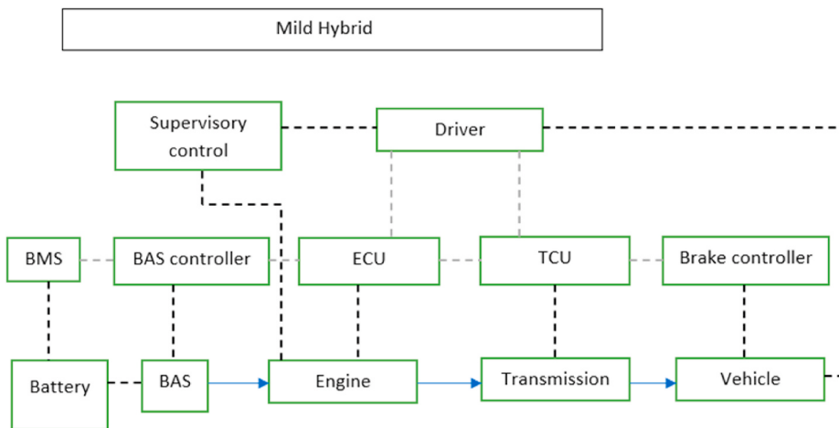
Fig. 2. Schematic vehicle model in GT Suite (with BAS).
