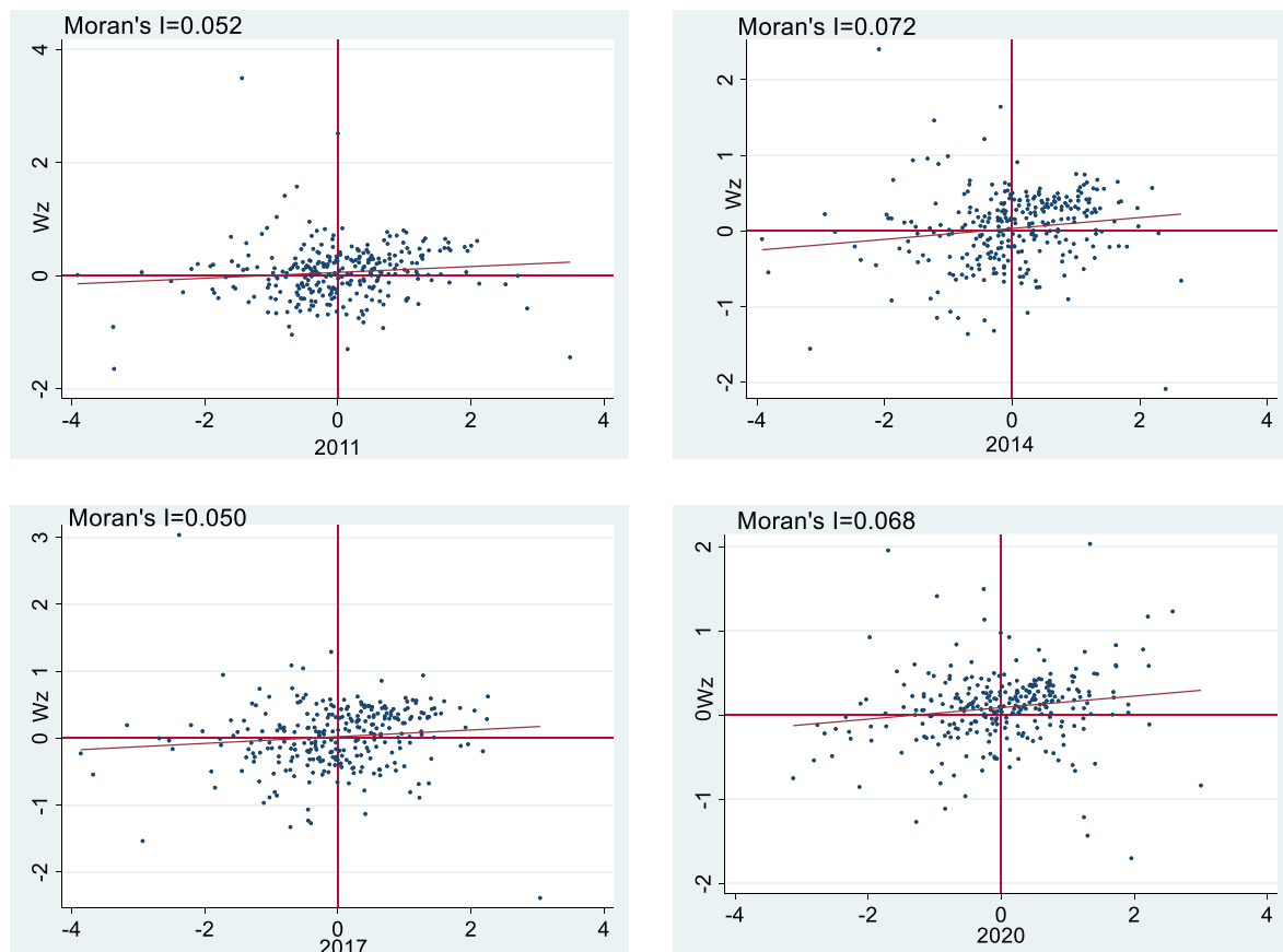
Fig. 2. Scatter graph of the local Moran's index of Isu in 2011, 2014, 2017, and 2020.
