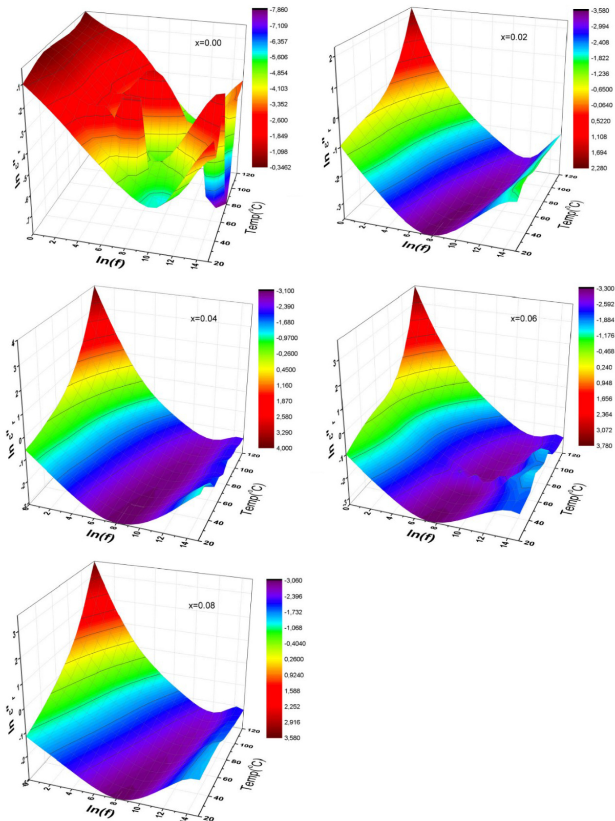
Fig. 6. 3D characteristic representations of dielectric loss of \text{BaNb}_x\text{Fe}_{12-x}\text{O}_{19} ( x \leq 0.08 ) HF as a function of frequency up to 3 MHz, and for temperatures up to 120 °C.
