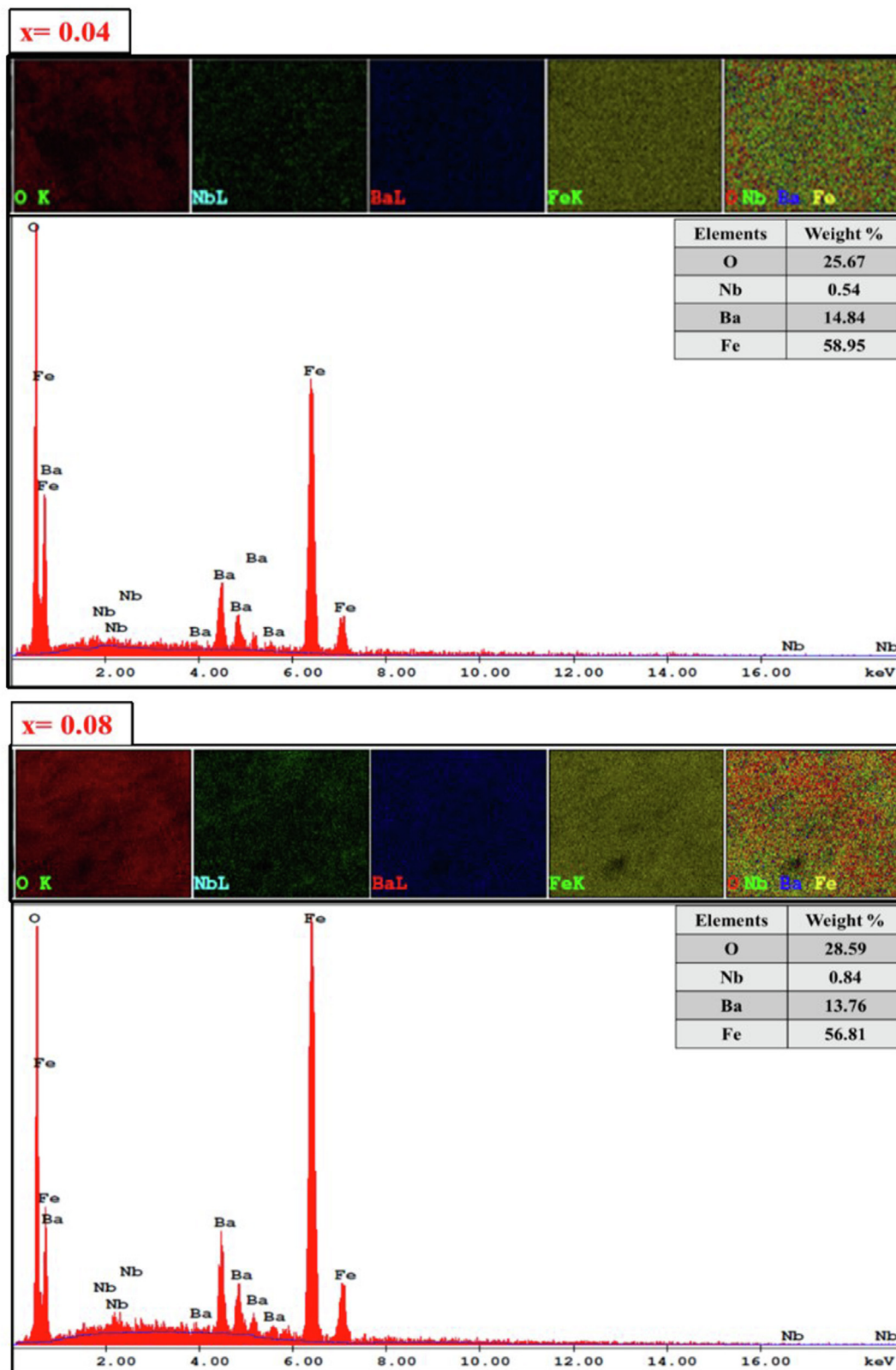
Fig. 3. EDX and elemental mapping of \text{BaFe}_{12-x}\text{Nb}_x\text{O}_{19} ( x = 0.04 and 0.08 ) HF's.
