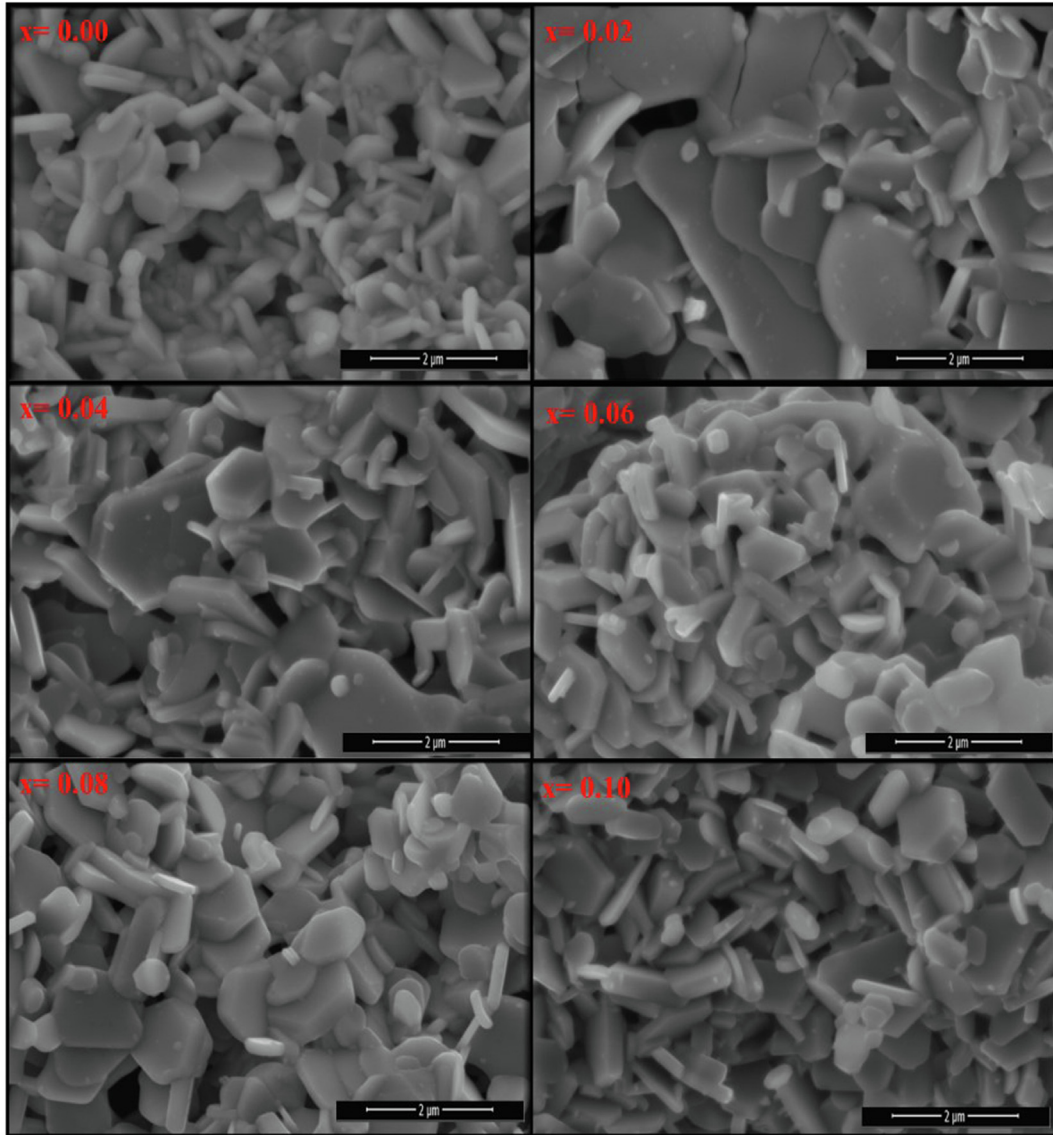
Fig. 2. FE-SEM images of \text{BaFe}_{12-x}\text{Nb}_x\text{O}_{19} ( x \leq 0.1 ) HFs.
