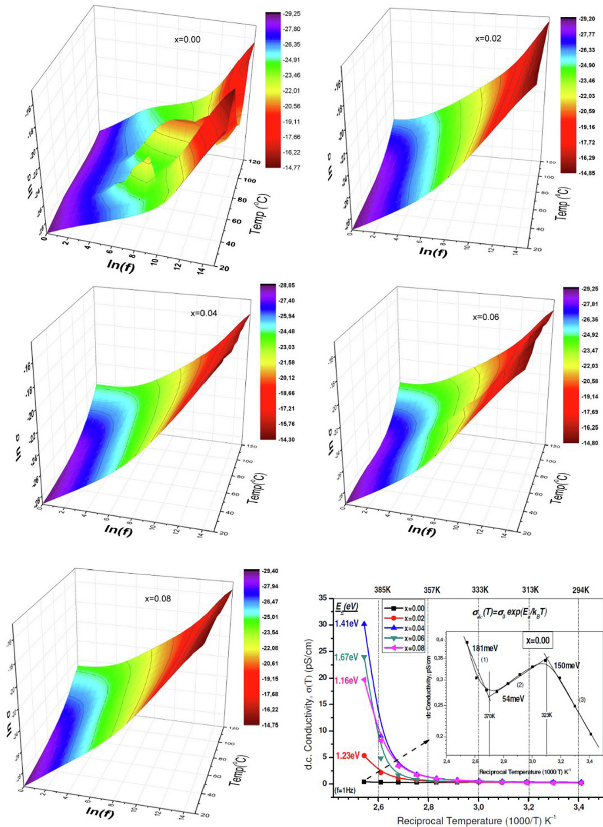
Fig. 4. 3D characteristic representations of ac conductivity of \text{BaNb}_x\text{Fe}_{12-x}\text{O}_{19} ( x \leq 0.08 ) HF's as functions of frequency up to 3 MHz, and for temperatures up to 120 °C. Last graph shows dc conductivity as a function of reciprocal temperature for some substitutional Nb ion ratios.
