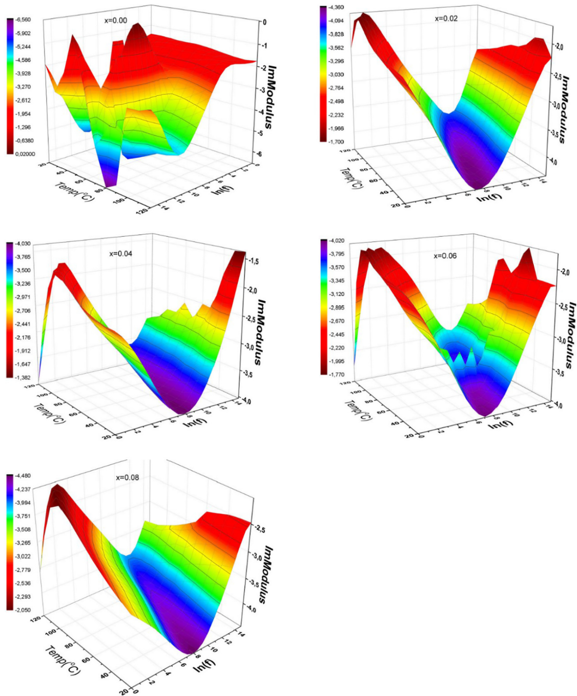
Fig. 9. 3D characteristic representations of dielectric imaginary modulus of \text{BaNb}_x\text{Fe}_{12-x}\text{O}_{19} ( x \leq 0.08 ) HF's as a function of frequency up to 3 MHz, and for temperatures up to 120 °C.
