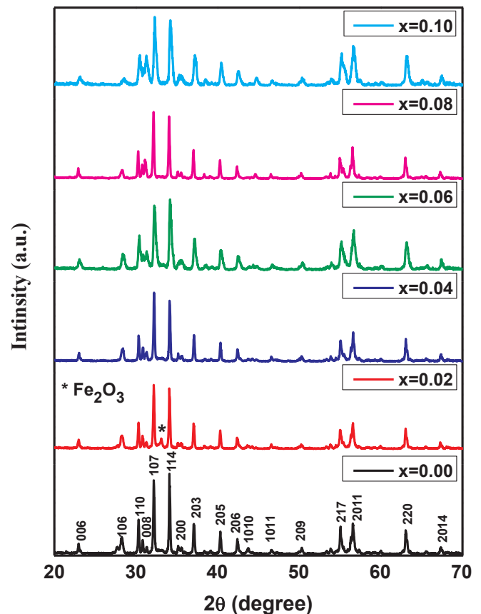
Fig. 1. XRD patterns for \text{BaFe}_{12-x}\text{Nb}_x\text{O}_{19} ( x \leq 0.1 ) HFes.
