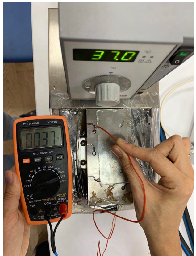
Fig. 1. Measuring the temperature of the artificial canal using a thermocouple.
