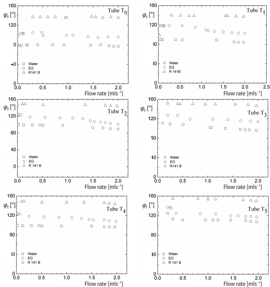
Figure 6. Effect of condensate flow rate on test tubes using water, ethylene glycol and R-141b as test fluids
