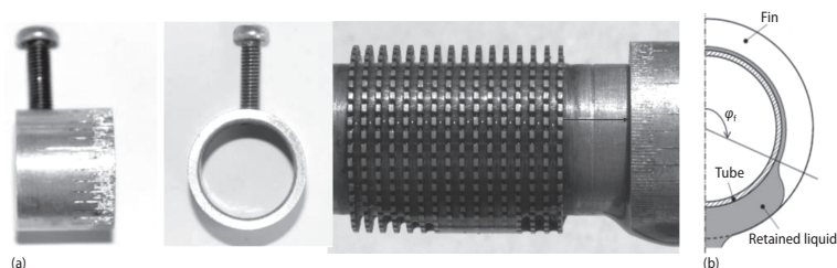
Figure 3. (a) Calibrated ring for the measurement of condensate retention angle, (b) condensate retention angle
