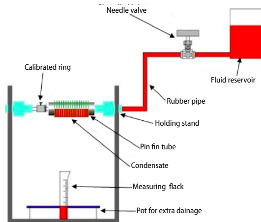
Figure 1. Schematic of Apparatus
