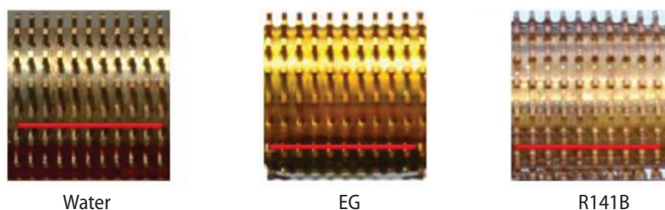
Figure 5. Photographs of test tube T5 with minimum flow rate (Lines show the retention angles) (for color image see journal web site)
