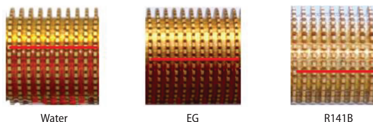
Figure 4. Photographs of test tube T0 with minimum flow rate (Lines show the retention angles) (for color image see journal web site)
