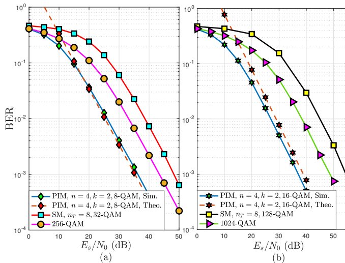
Fig. 4. Performance comparisons of SM, and traditional QAM systems for (a) 8 bpcu (b) 10 bpcu.
