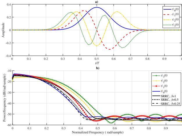
Fig. 1. Different Hermite-Gaussian pulses (a) with L = 127 in time-domain (b) bandwidth comparison with SRRC in frequency-domain.
